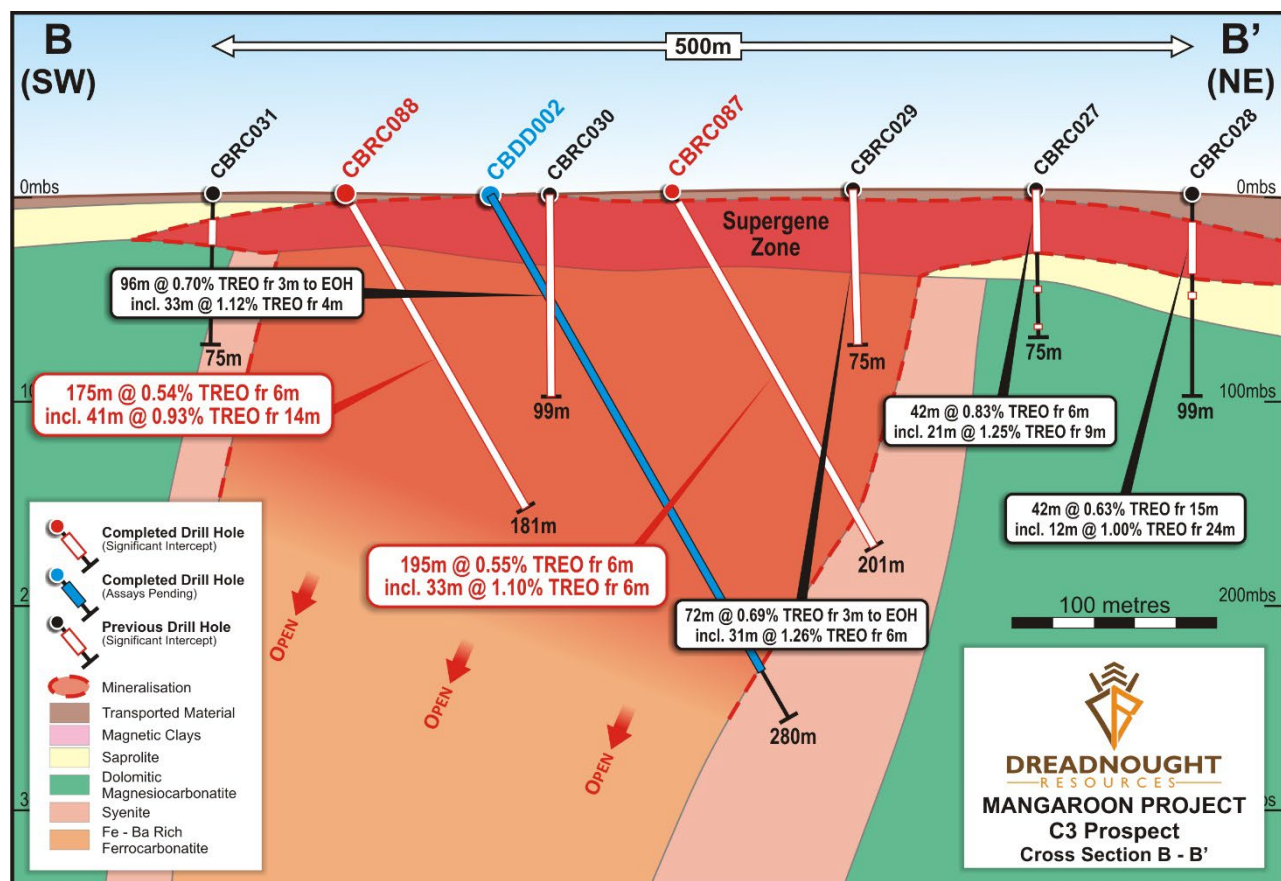
Figure 5: Cross section through C3 highlighting the mineralised intercepts (red), initial shallow vertical holes (black) and a diamond hole (blue).
