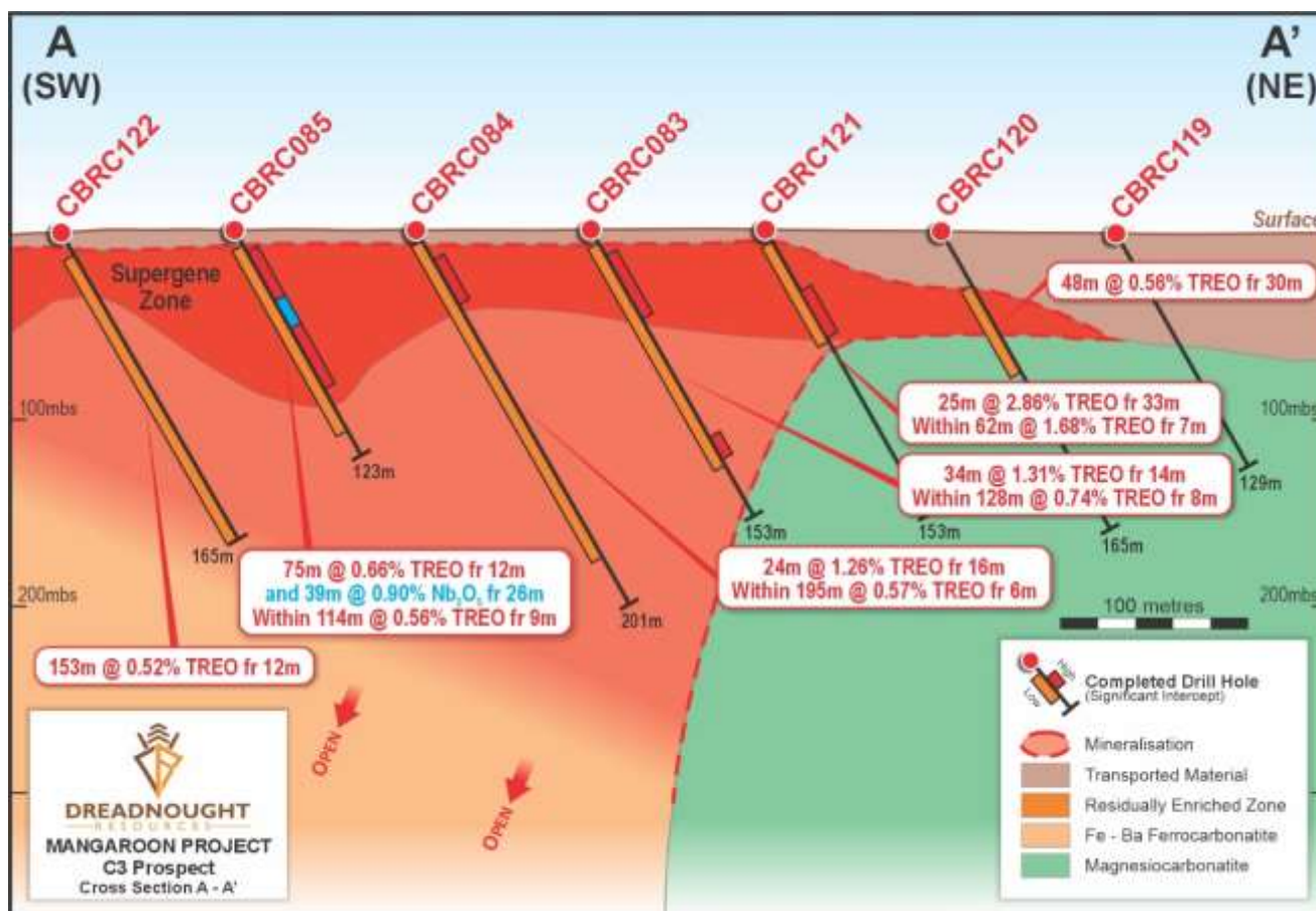
Figure 4: Cross section A-A' through C3 showing recent infill holes (red) with high grade REE and niobium mineralisation within the supergene zone and low grade REE mineralisation within the Ferrocarnatite.
