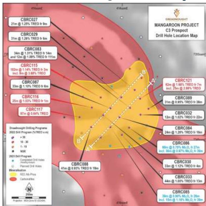
Figure 3: Plan view of the ~400m x 400m high grade rare earth and niobium zone at C3. Mineralised intercepts and planned holes are featured over a greyscale magnetic image (RTP IVD).
