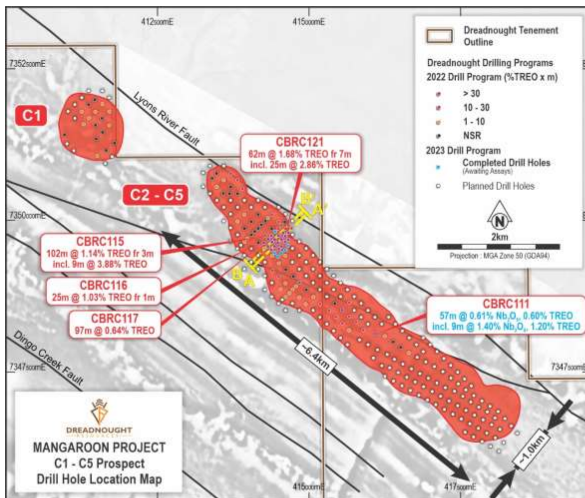
Figure 2: Plan view of the C1-C5 carbonatites over a greyscale magnetic image (RTP IVD) showing drill hole locations colored by %TREO x the mineralised interval. The shallow, high grade rare earth and niobium zones at C3 are apparent and featured in Sections A
