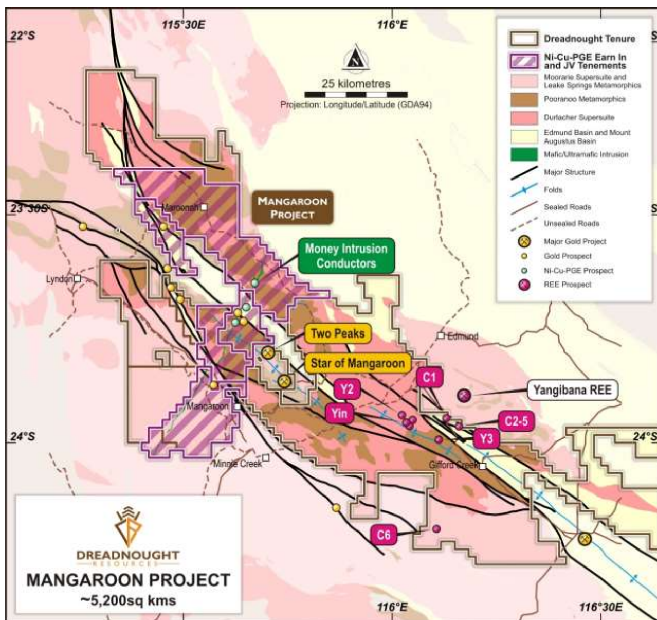
Figure 5: Plan view map of Mangaroon showing the location of the FQM Earn-in and 100% Dreadnought ground in relation to major structures, geology and roads.
