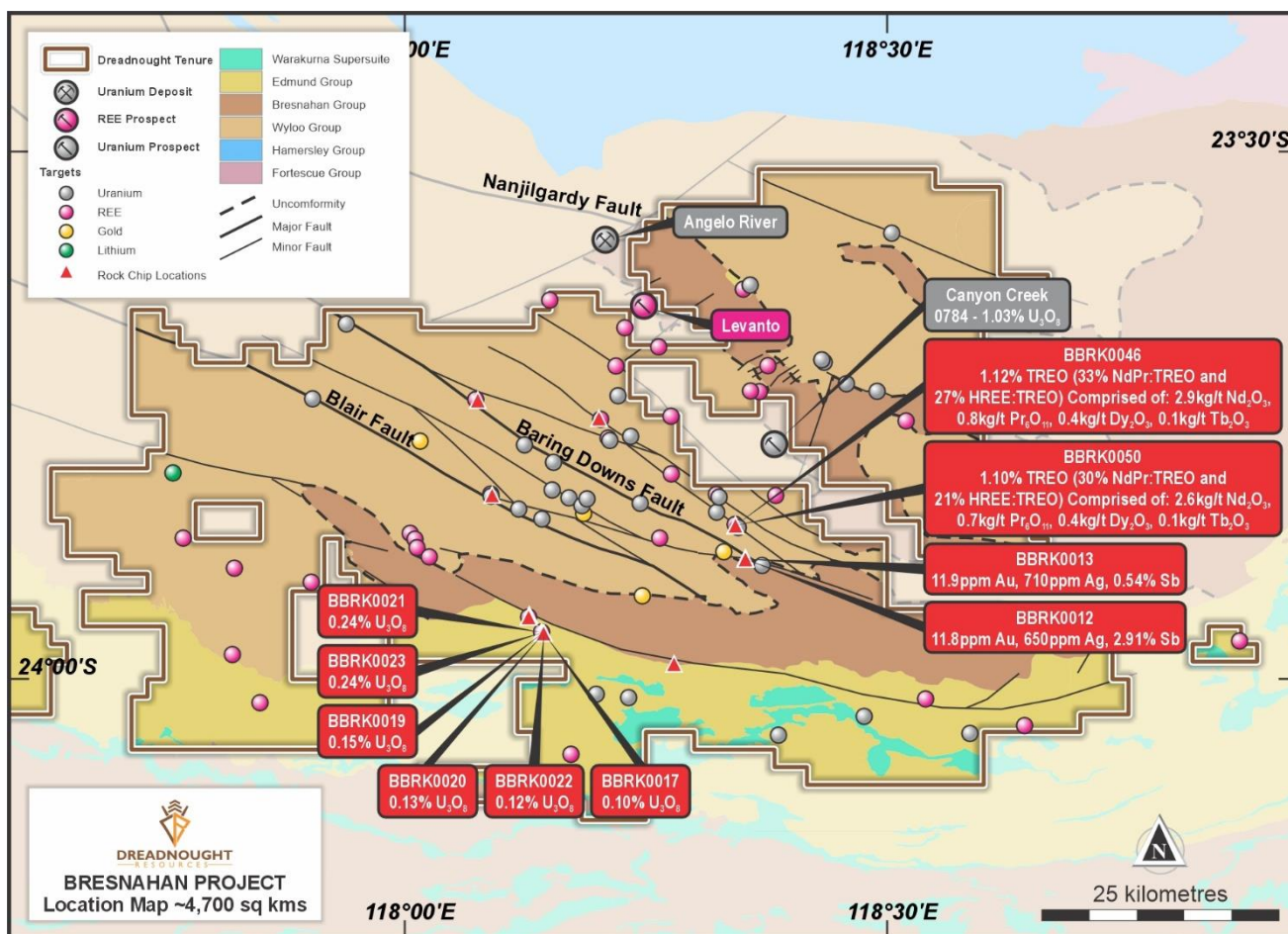
Figure 2: Plan view map of Bresnahan showing the location of mineralised rock chips and prospects in relation to the major structures and the Bresnahan-Wyloo unconformity.
