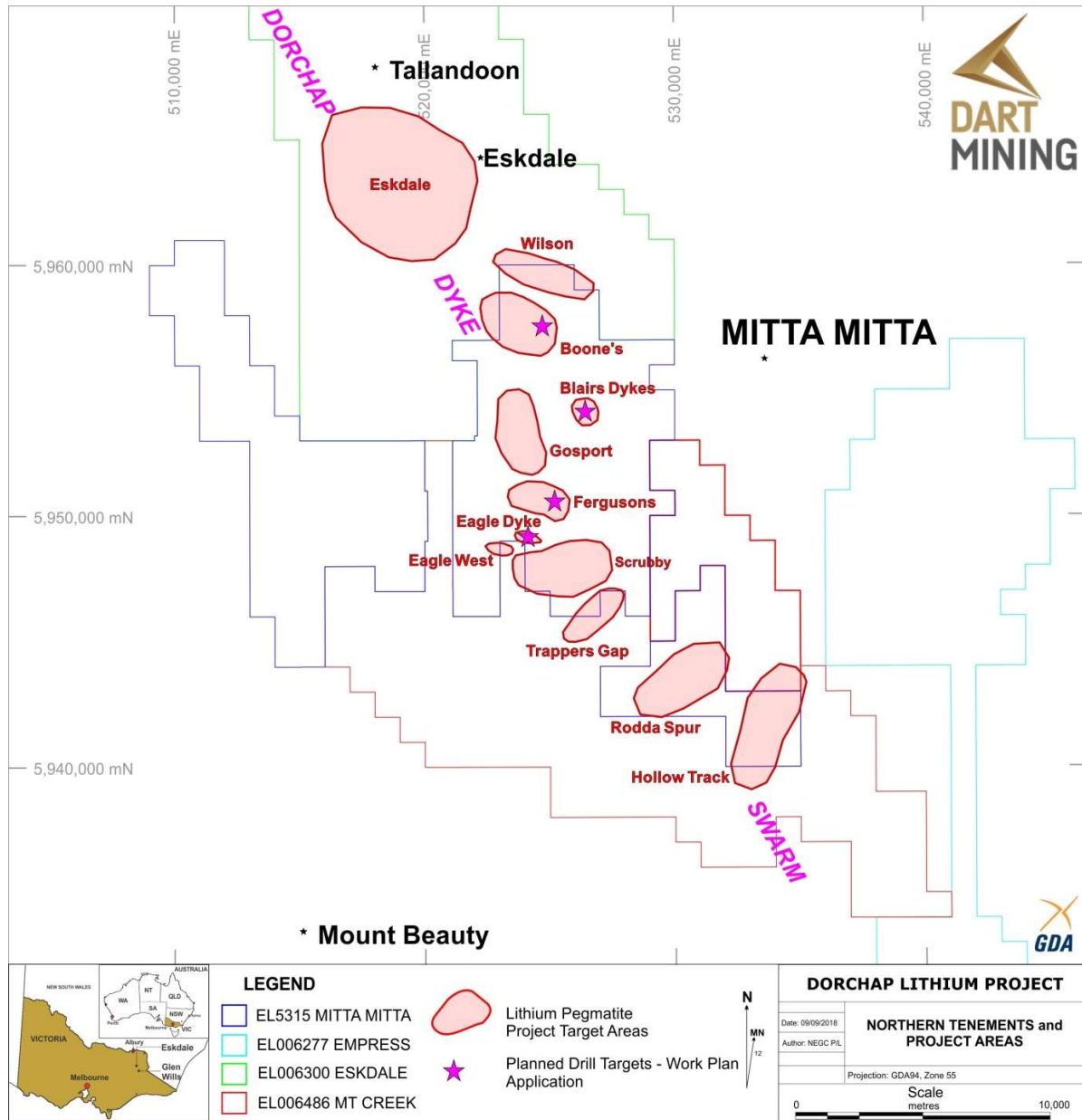
Figure 1. Dorchap Lithium Project – Tenements and Pegmatite Target areas (Northern Dorchap Dyke Swarm).
