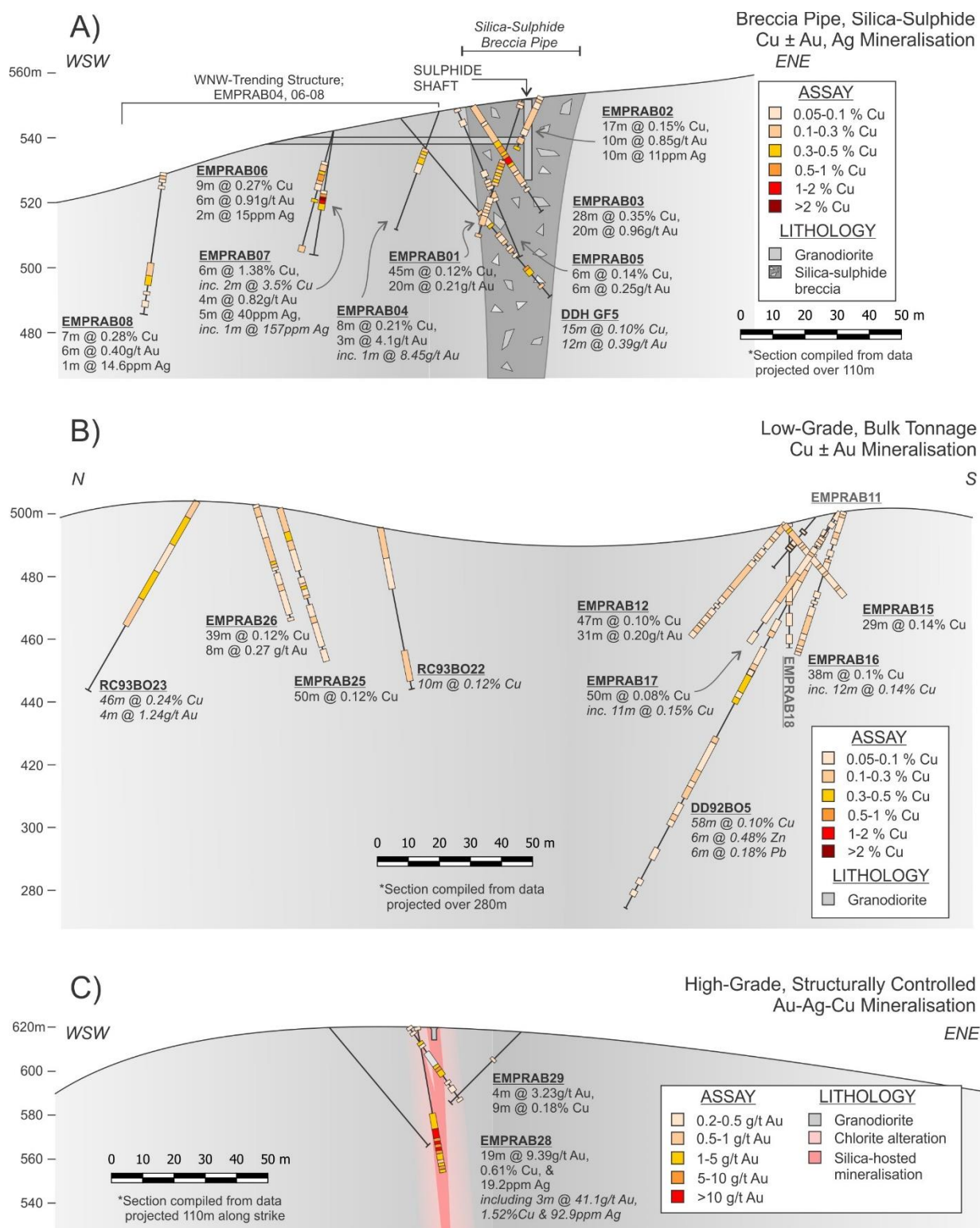
Figure 2: Cross-sections displaying preliminary geological interpretation of selected transects at Granite Flat, demonstrating the diversity and complexity of mineralisation styles encountered during drilling, including silica-sulphide mineralisation of breccia pipes (A), broad, low-grade Cu-Au mineralisation (B), and narrow, high-grade Au-Ag-Cu mineralisation (C). Drill results for historic drill holes DD92BO5, RC93BO22, RC93BO23 and DDH GF5 obtained from open file GSV reports (as reported in Dart ASX October 2020 ).
