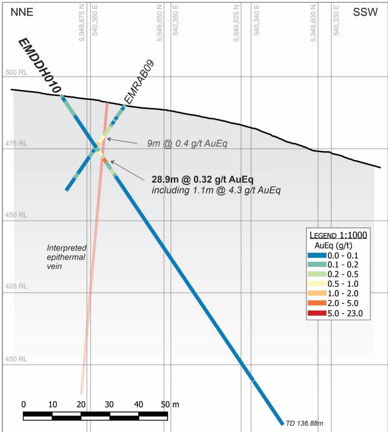
Figure 9 – Cross section of drill hole EMDDH010 showing all mineralised intercepts. RAB drilling results from DTM ASX March 2021 .
