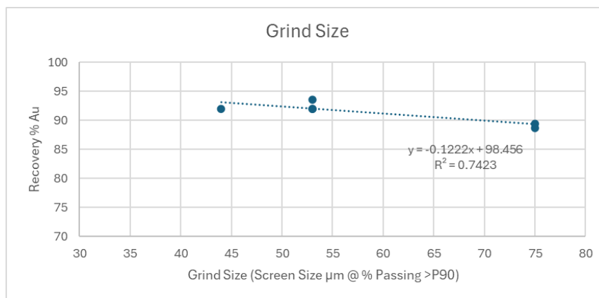
Figure 17 Leach Recovery vs Grind Size
