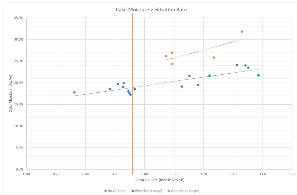
Figure 30 Jord Filter Results
