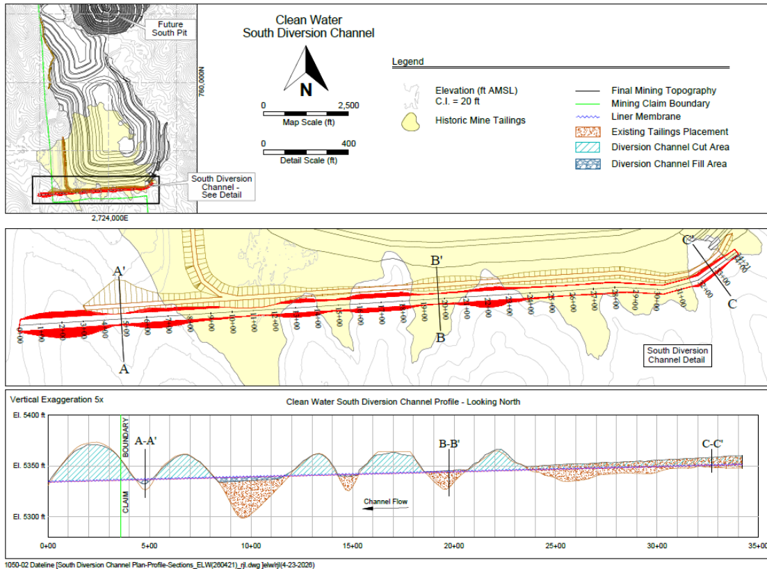
Figure 51 Clean Water Diversion Channel
