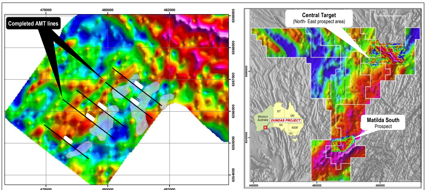
Figure 4: Left: Central Target showing location of planned AMT lines over interpreted SkyTEM conductors (shaded polygons), underlying image is gravity. AMT Lines 11000 and 12250 have been completed
