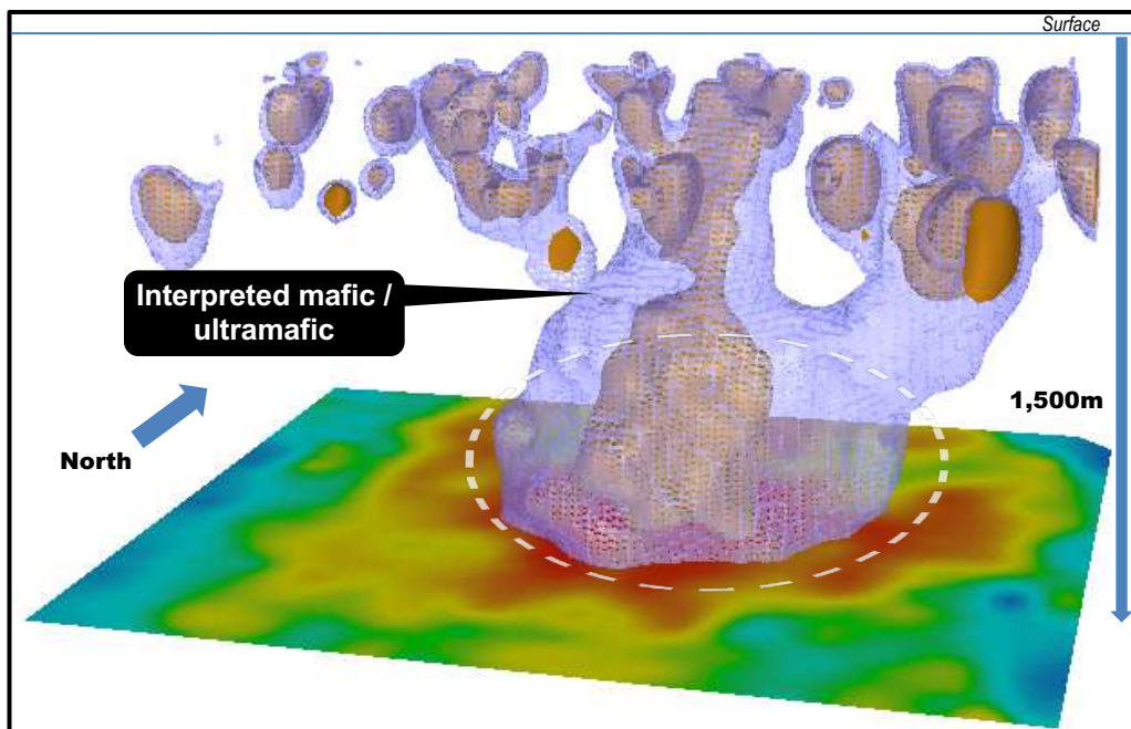
Figure 3: Matilda South: 3D gravity model (brown = 3.4\text{t/m}^3 , purple = 3\text{t/m}^3 ) placed above gravity anomaly
