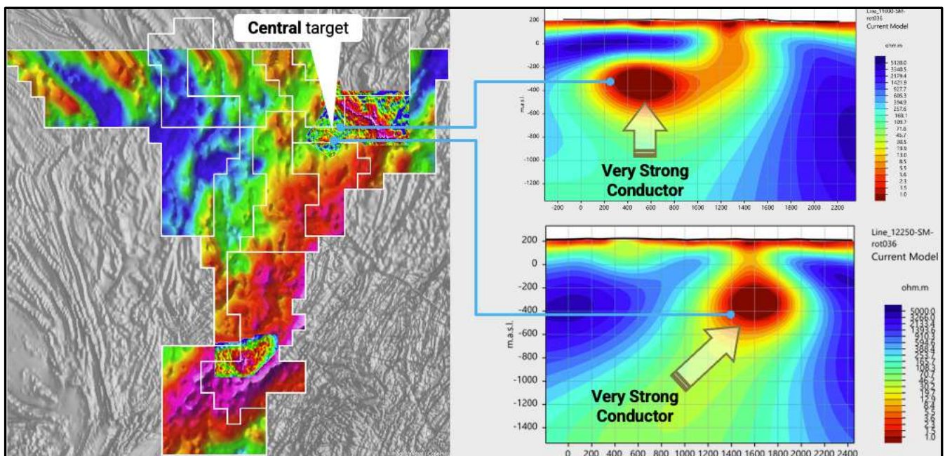
Figure 3: Central AMT anomalies (low resistivity, high conductivity), as announced on 16 March 2022
