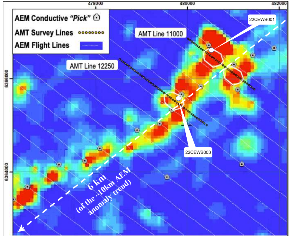
Figure 4 180m SkyTEM AEM Depth Slice (channel 41). White circled areas outline the very low resistivity AMT anomalies
