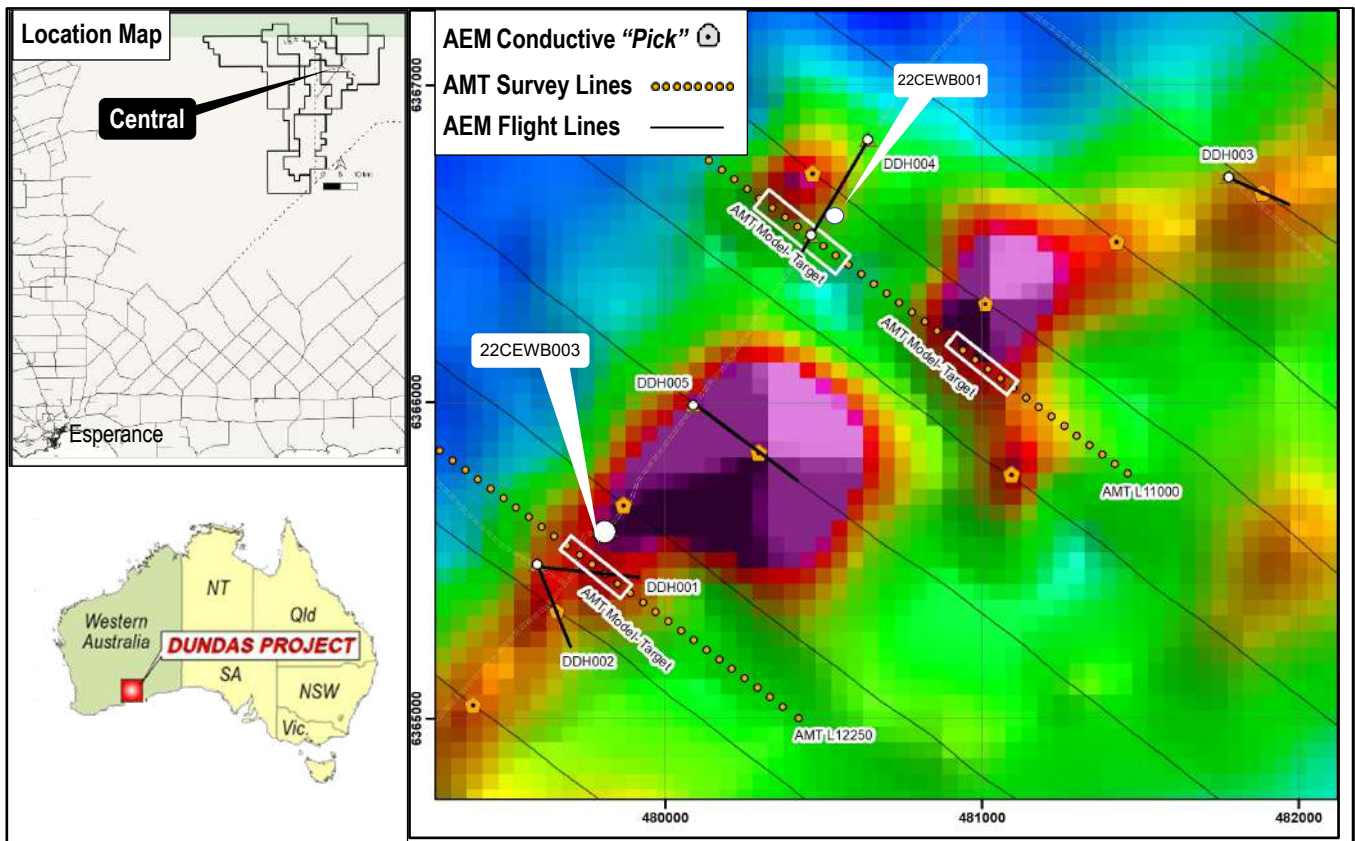
Figure 2: Late-time (B Field channel 41), aerial electromagnetic (AEM) anomaly trend at Central target with AMT model drill targets in white boxes (lines 12250 and lines 11000) and locations of planned drill holes DDH001 to DDH005 marked.
