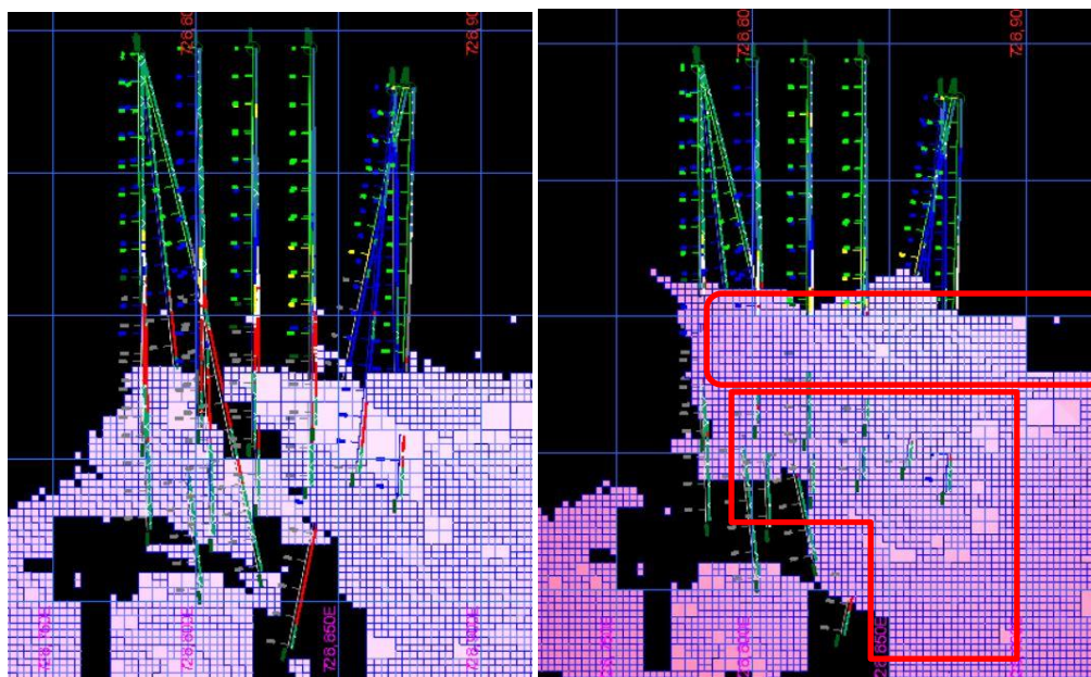
Figure 3: Indicated Resource Blocks: Image on the left shows the Indicated Resource blocks within the 2016 Resource estimate. The image on the right shows the area promoted to Indicated Resource, the main areas promoted are defined by red outlines. The image looks to the north with only holes from the 2017 program shown.
