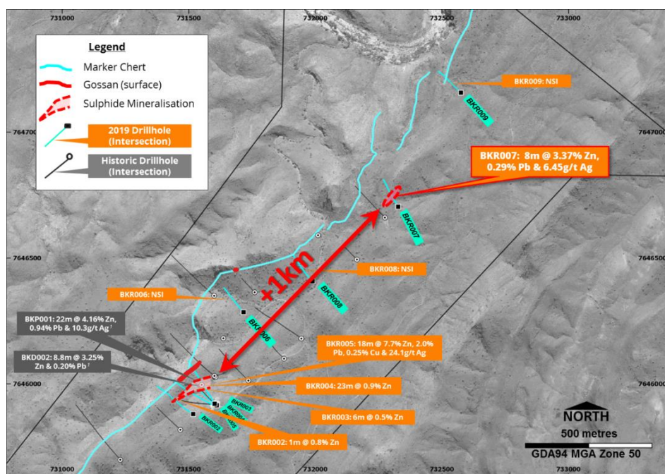
Image 5: Plan view of Breakers exploration drilling
