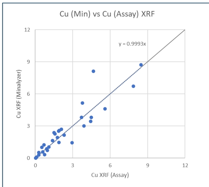
Figure 6: Cu-grades of selected calibration samples.
