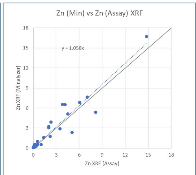
Figure 7: Zn-grades of selected calibration samples.
