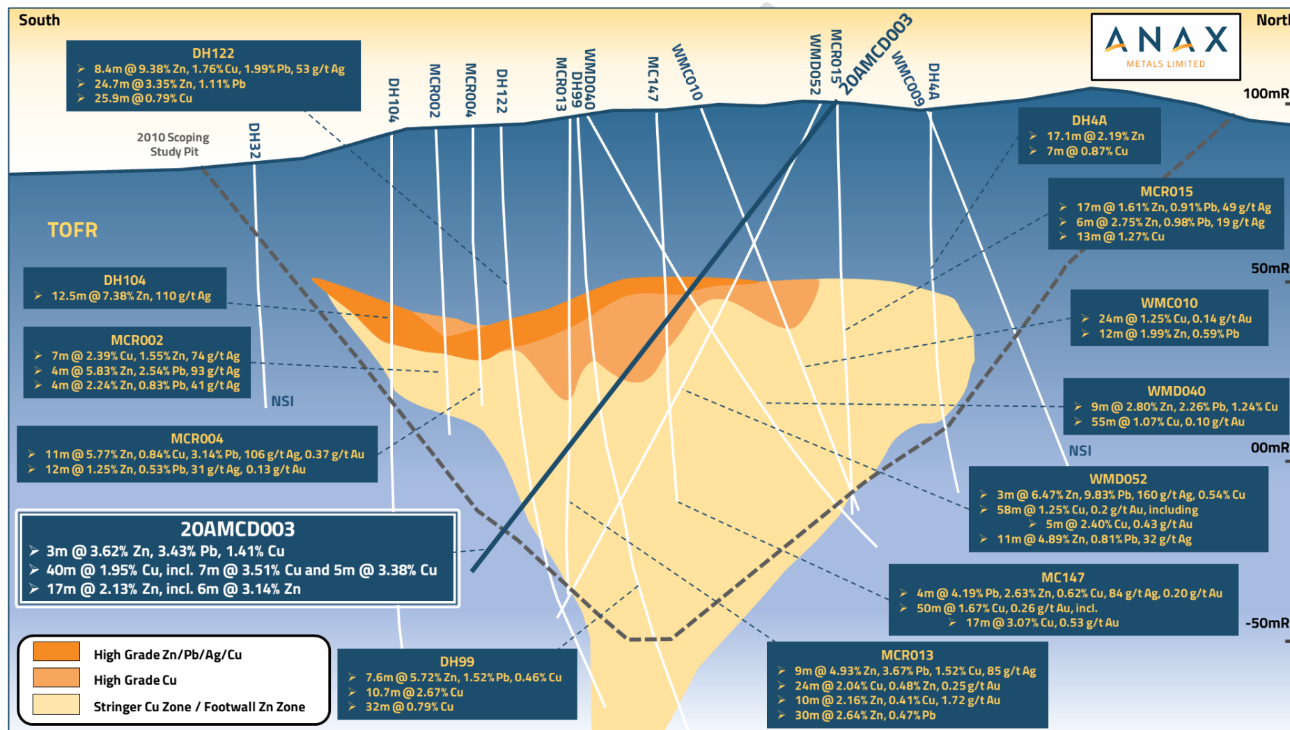
Figure 5: Mons Cupri Cross Section through 583,860mE showing 20AMCD003 and select previous drill holes. Note: A number of holes have been omitted from the section for ease of display; only the most significant intervals are displayed - for a full list of intersections refer to Table 3 and Table 10.
