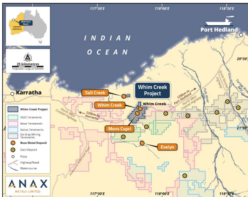
Figure 9: Whim Creek Project Location
