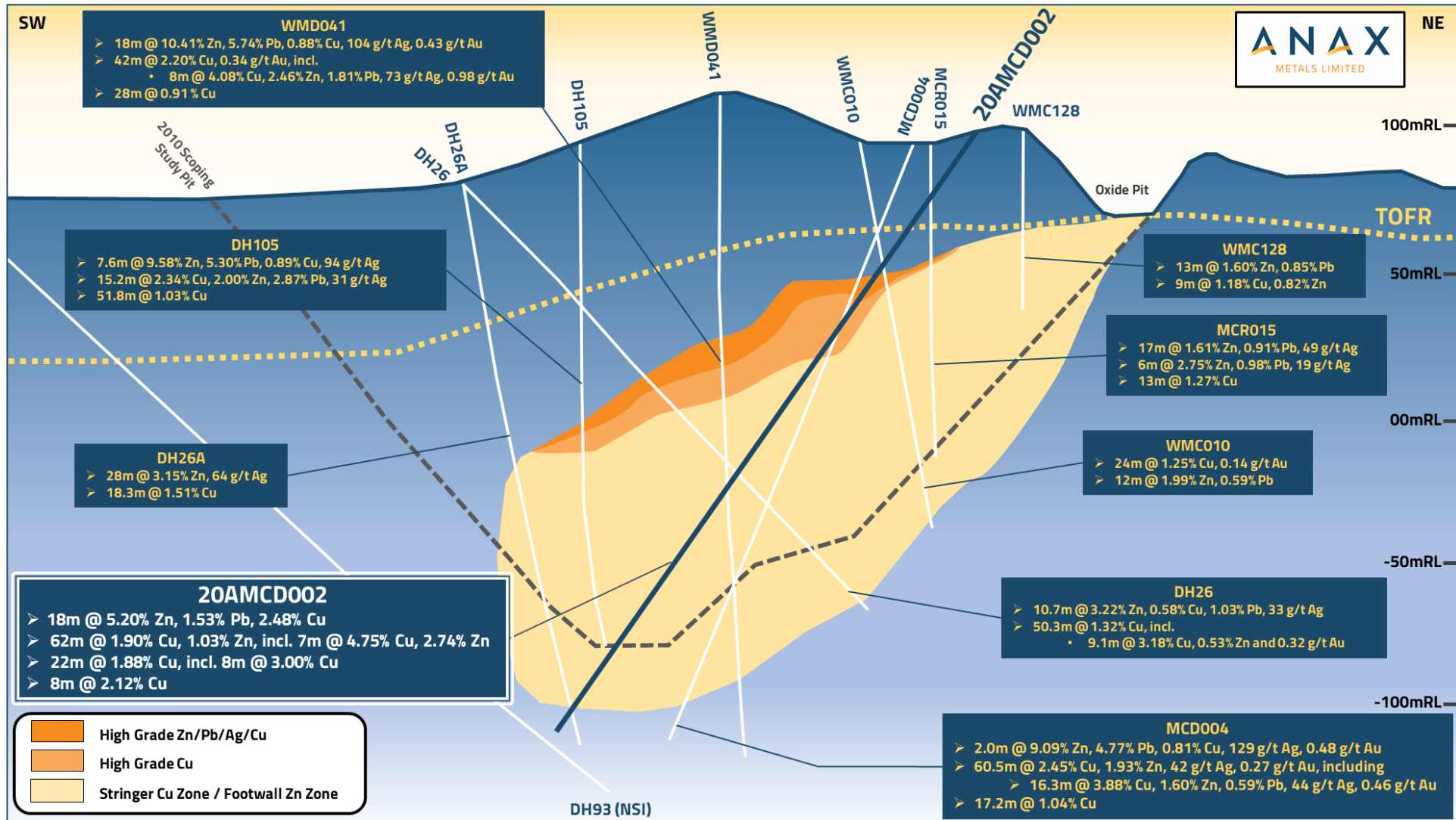
Figure 3: Mons Cupri Oblique Section showing 20AMCD002 and select previous drill holes. Note: A number of holes have been omitted from the section for ease of display; only the most significant intervals are displayed - for a full list of intersections refer to Table 2 and Table 10.
