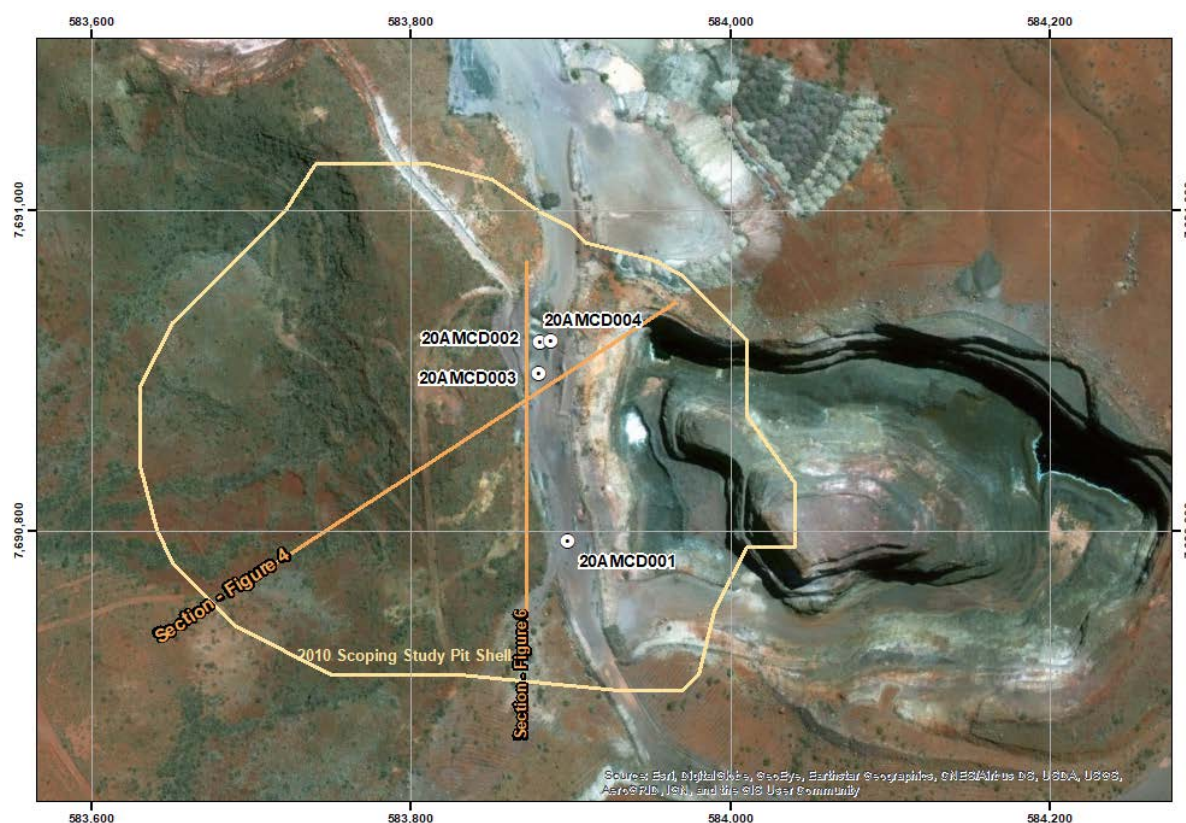
Figure 10: 2020 Anax Drilling and Cross Section Locations – Mons Cupri
