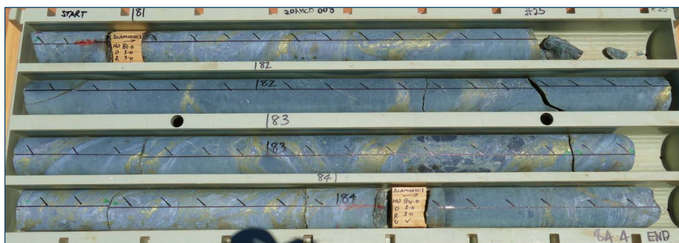
Figure 4: Stringer and semi-massive sulphide chalcopyrite mineralisation in 20AMCD003.
