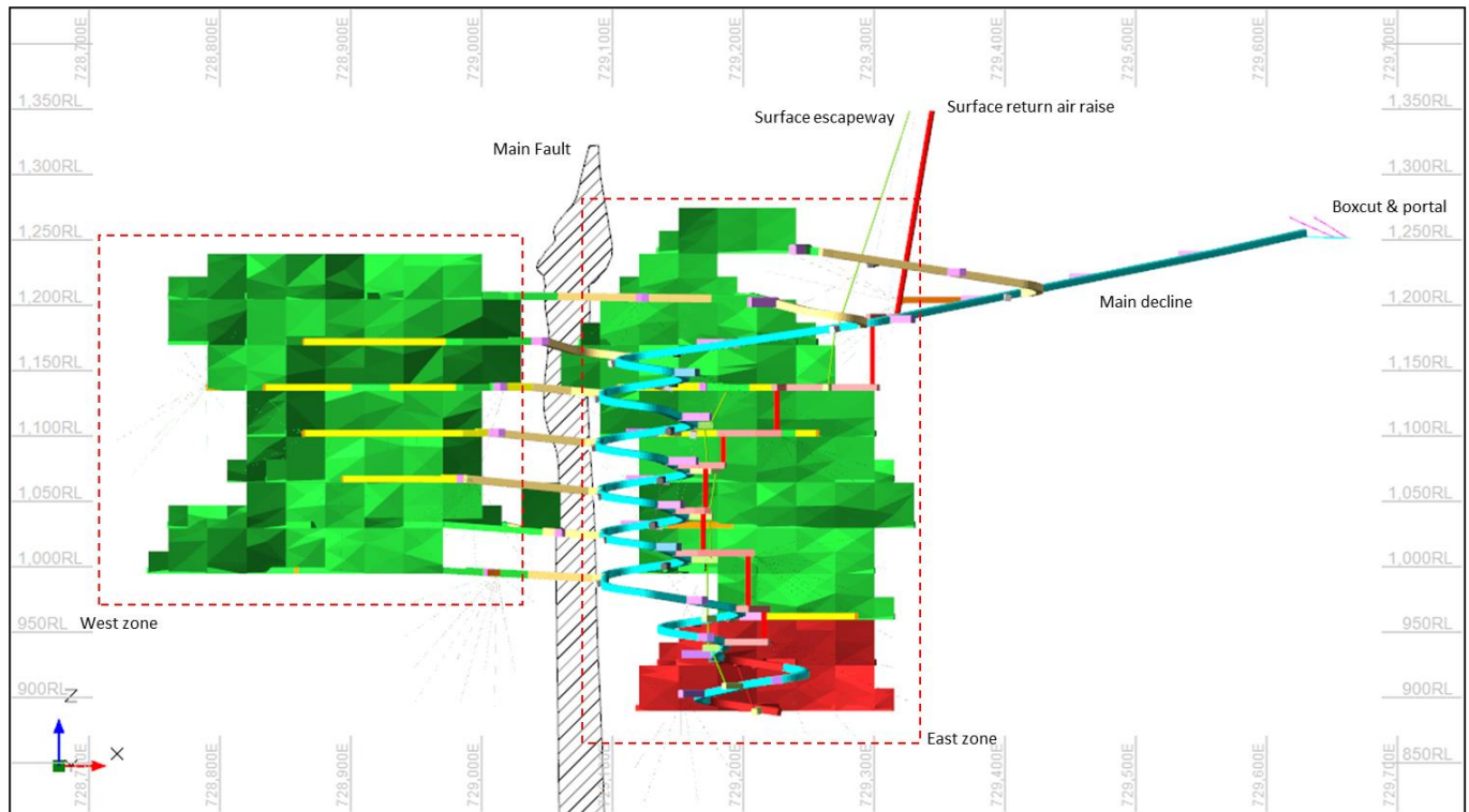
Figure 5 Sulphur Springs's mine design (looking north)
