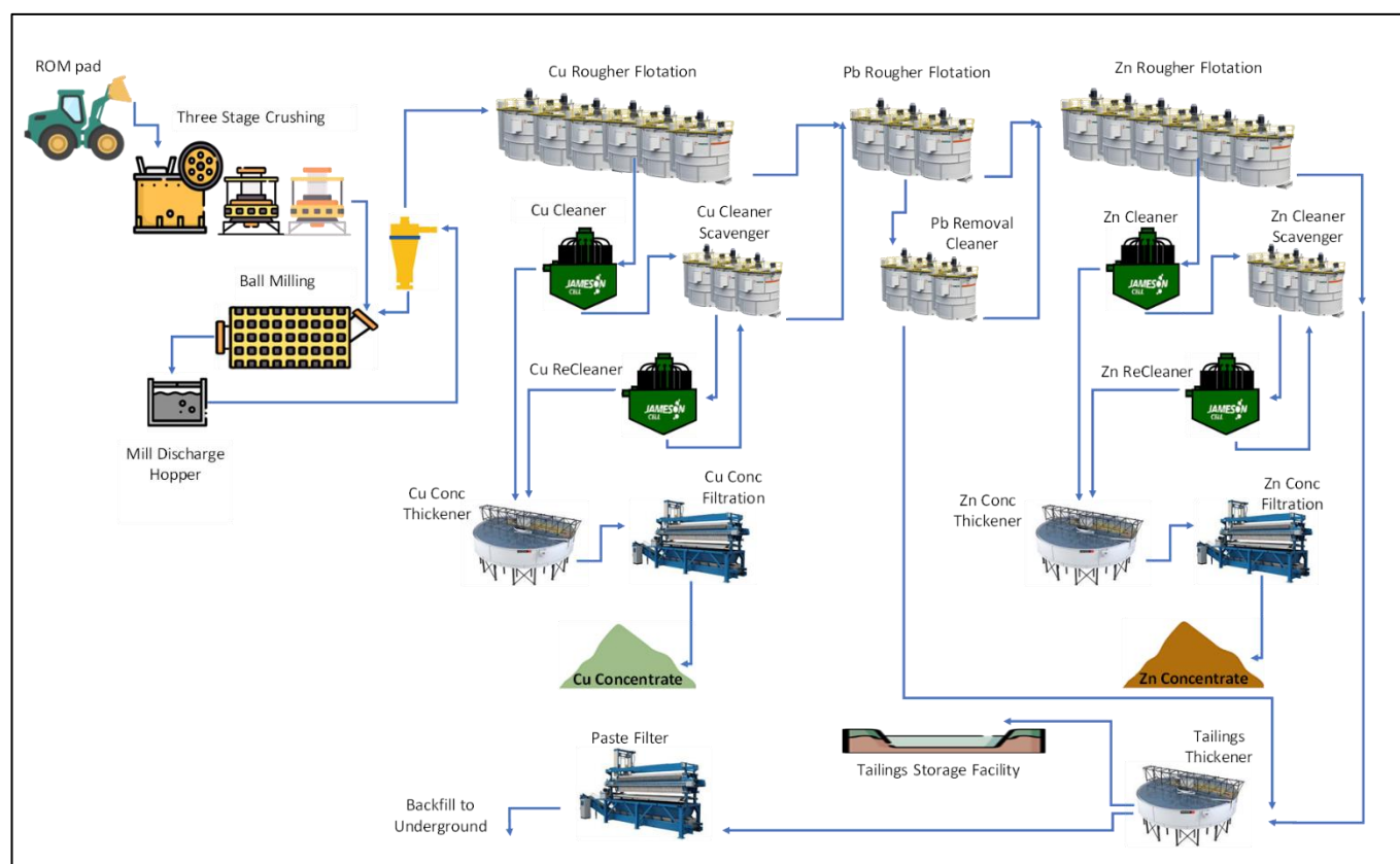
Figure 8 Updated Sulphur Springs Process Flowsheet
