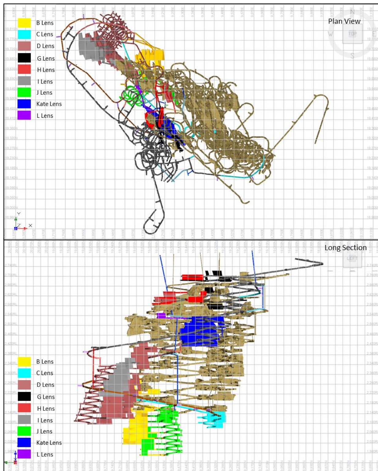
Figure 8: Mine plan
