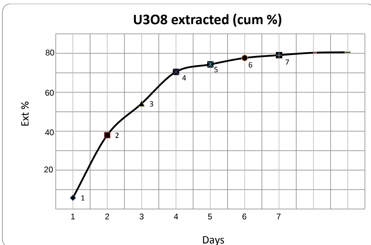
Graph 1: Uranium Recovery Curve
