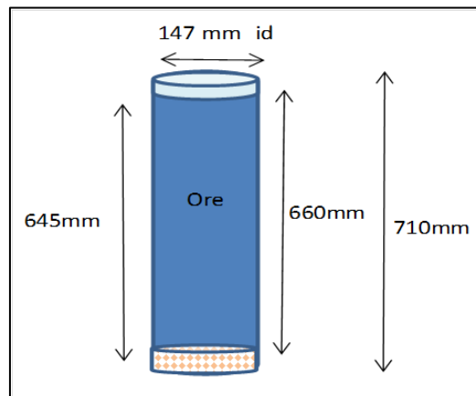
Figure 1: Column Dimensions
