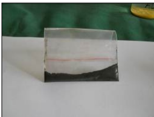
Photograph 10 – \text{U}_3\text{O}_8
