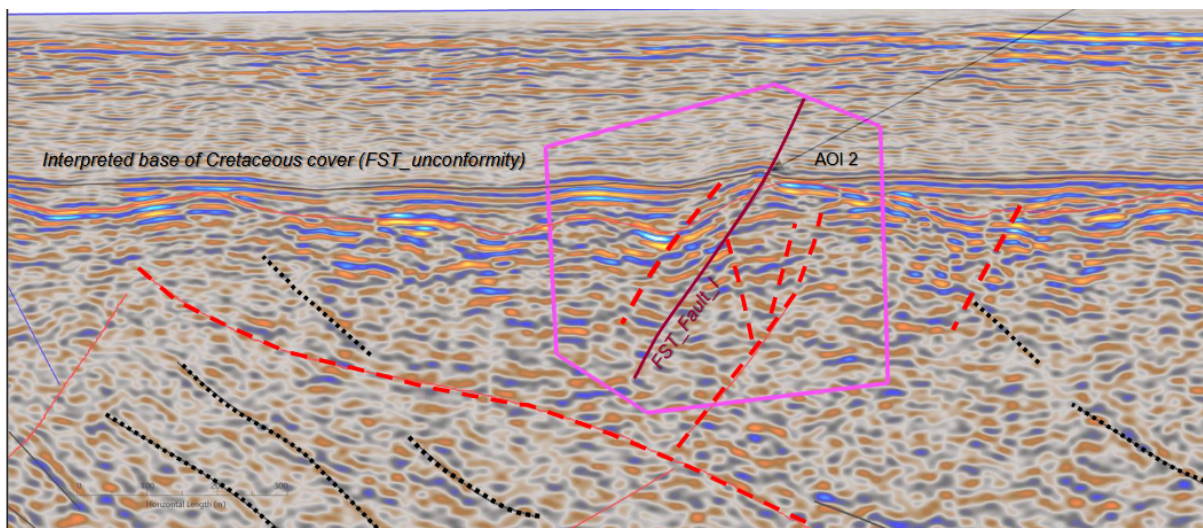
Figure 5: Cross-section of a 2D reflection seismic line showing an interpreted reverse fault.
