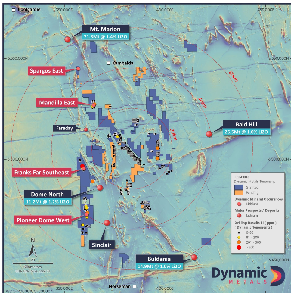
Figure 3. Dynamic's Widgiemoooltha Project tenements with key lithium projects and prospects
