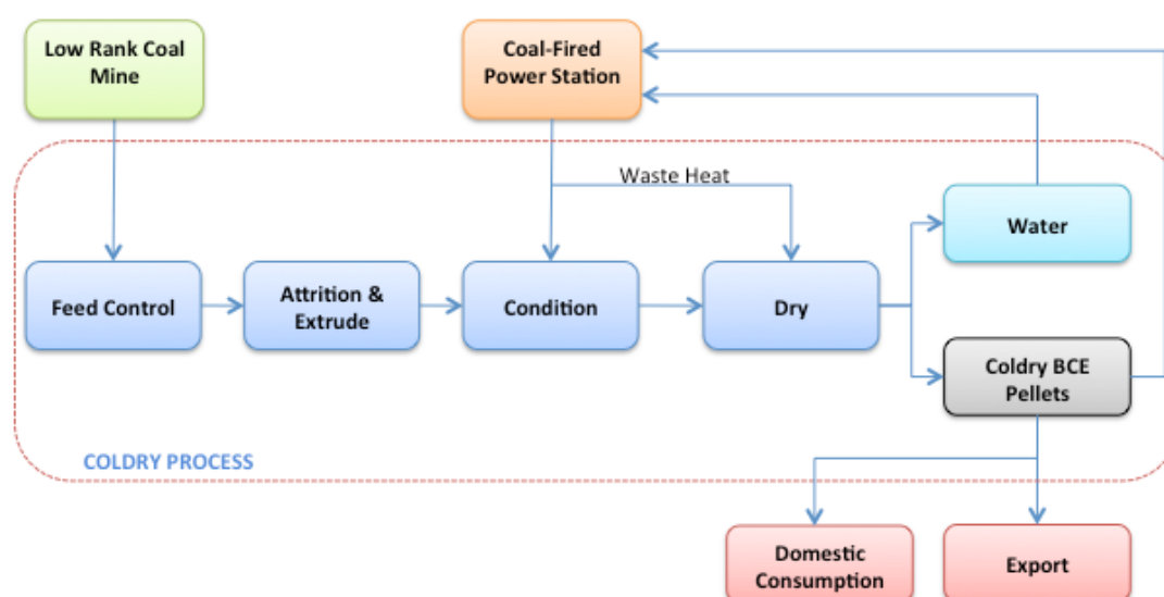
Figure 1: Coldry Process
