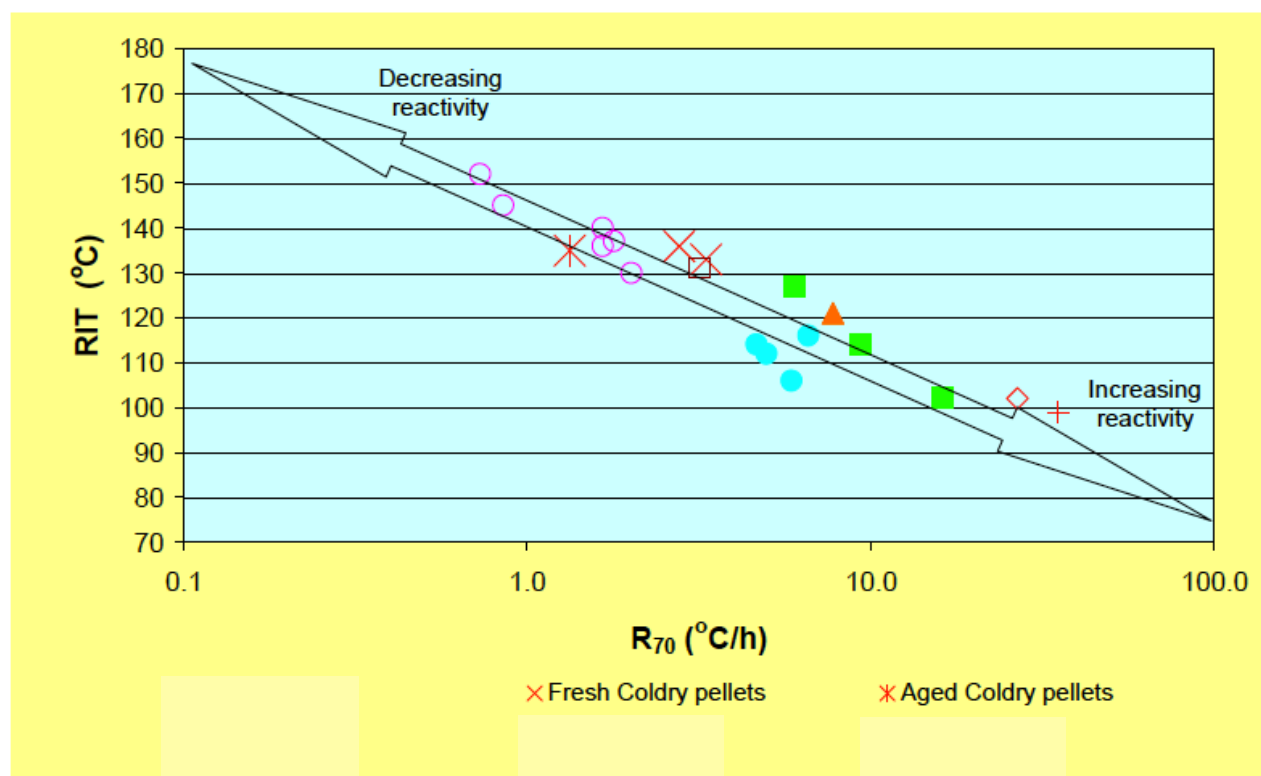
Figure 2 – Relative Ignition Temperature vs. R 70 (rate of self heating)
