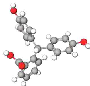
Complex organic hydrocarbons
