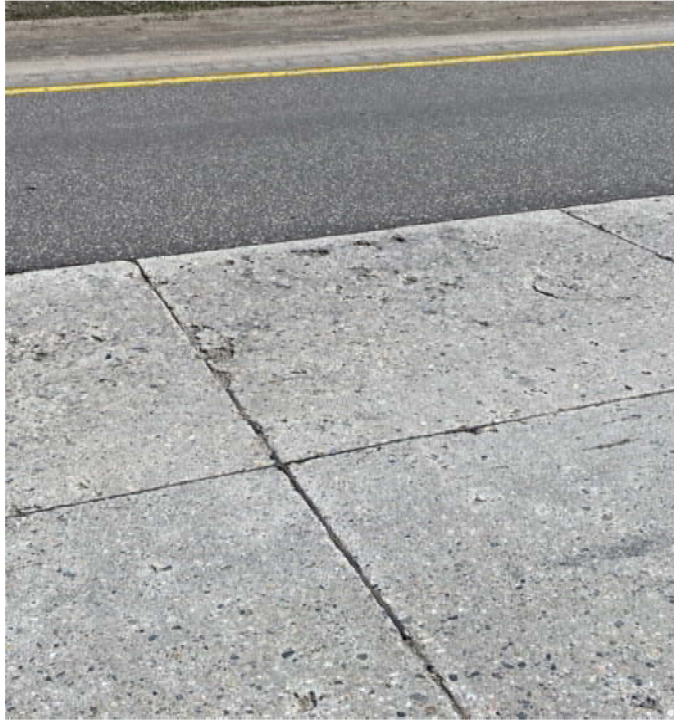
Figure 2 Mid-Section- Reference Slab -12 months Severe Surface Damage, Joint Rot, Pitting, Pop Outs
