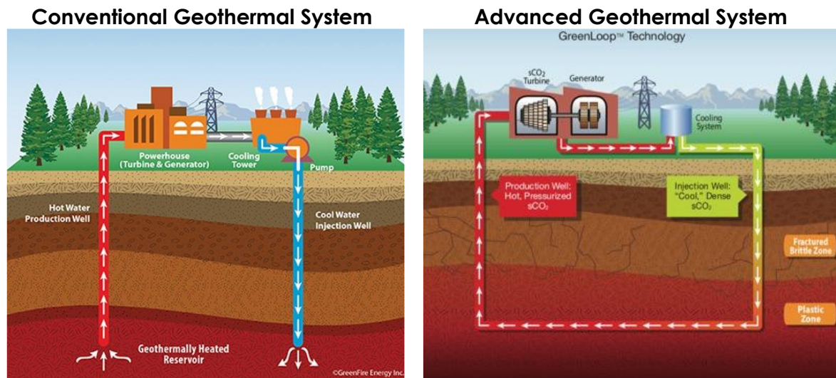
Figure 2 – Next Generation Geothermal Systems overcome location restrictions 7
