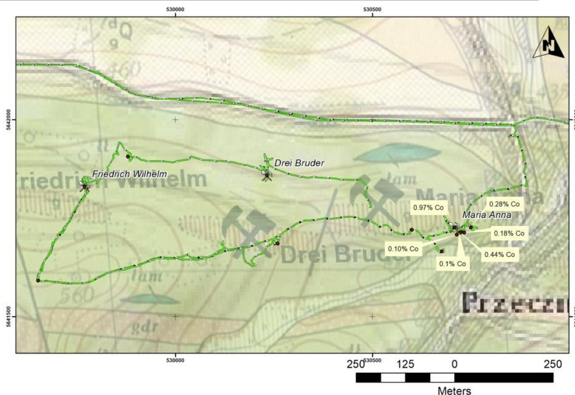
Figure 9: Geological map and sample locations around the Maria Anna cobalt mine.
