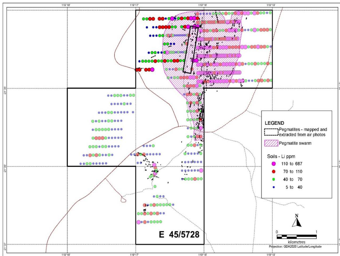
Figure 5: Soil Lithium geochemistry. Pre-existing soils results faded.
