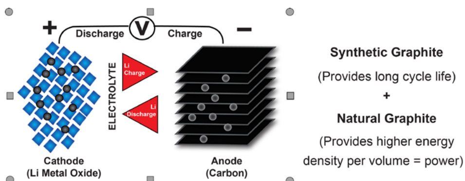
Figure 1 LiB Battery showing graphite anode (referenced and after Handbook on Rechargeable Batteries, 3 rd Edition)
