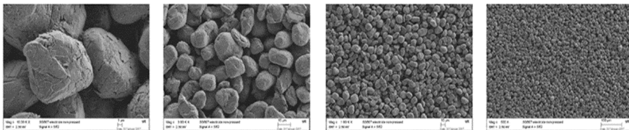
Image: Epanko spherical graphite at 10k, 3k, 1k and 500x magnification
