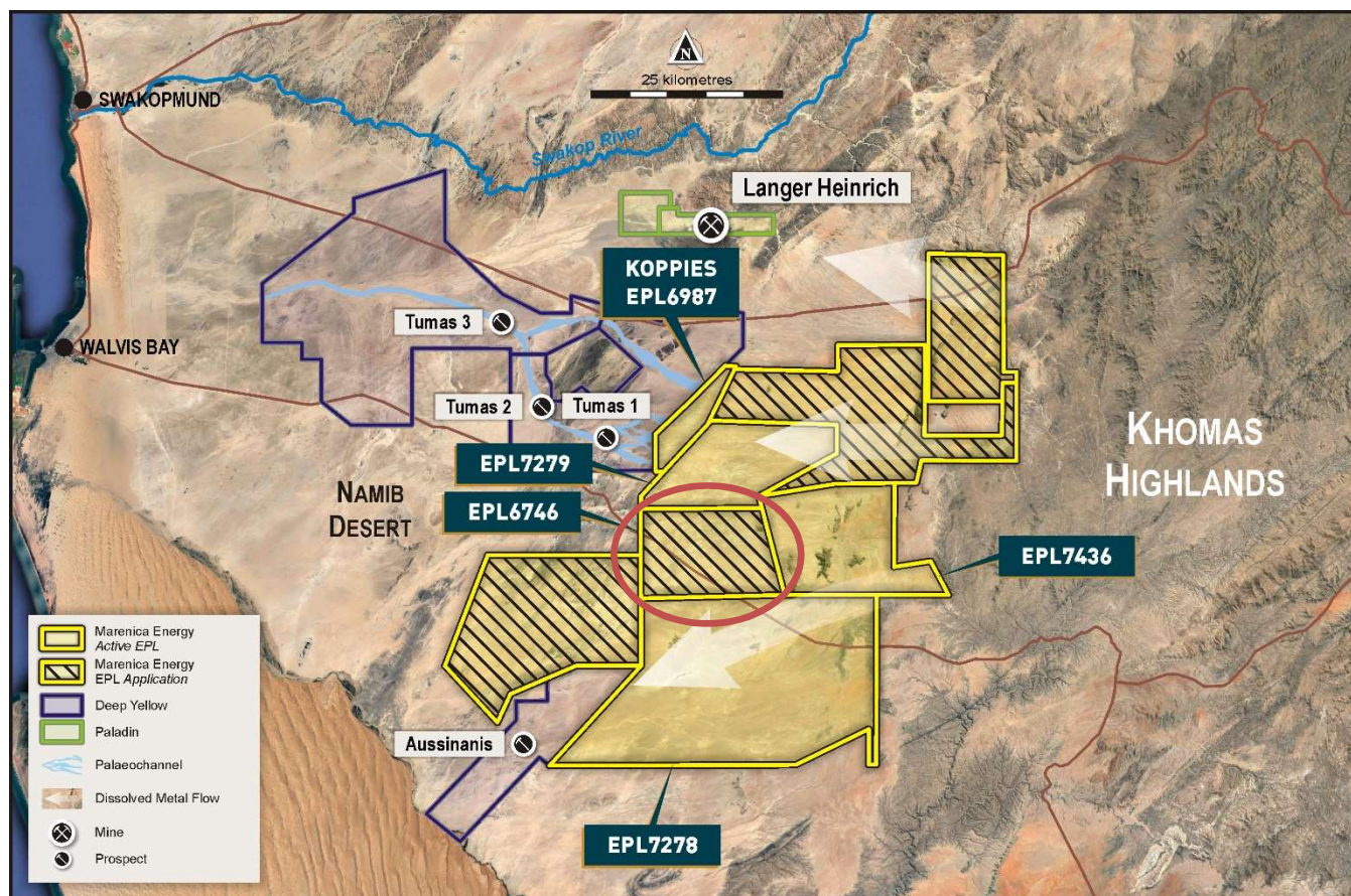
Figure 1 Location of EPL 6746 in the Namib Desert, Namibia.
