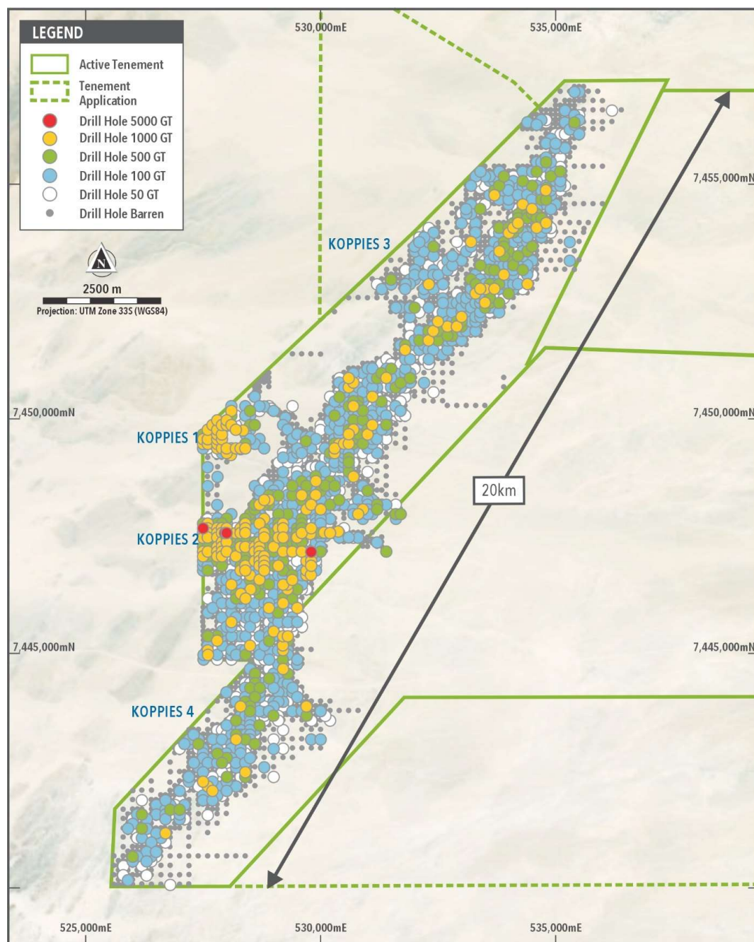
Figure 1 Koppies Drill Collar Locations & Grade Thickness
