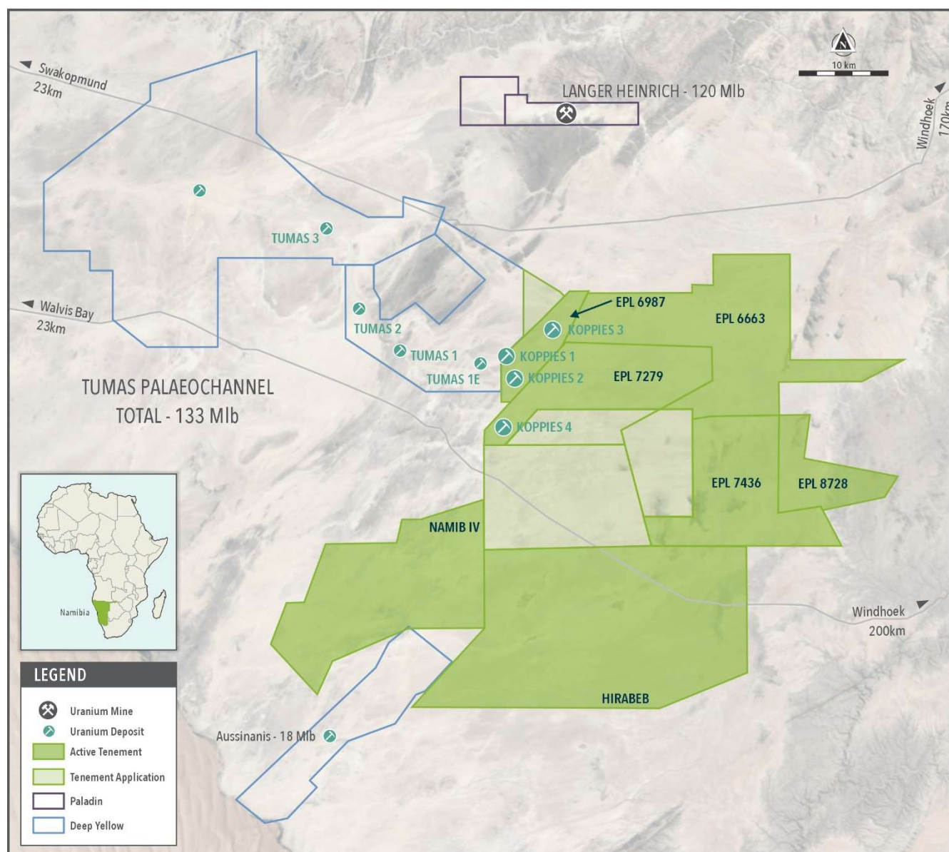
Figure 2 Location of Koppies with Respect to Elevate Uranium's Tenement Holding in the Namib Area
