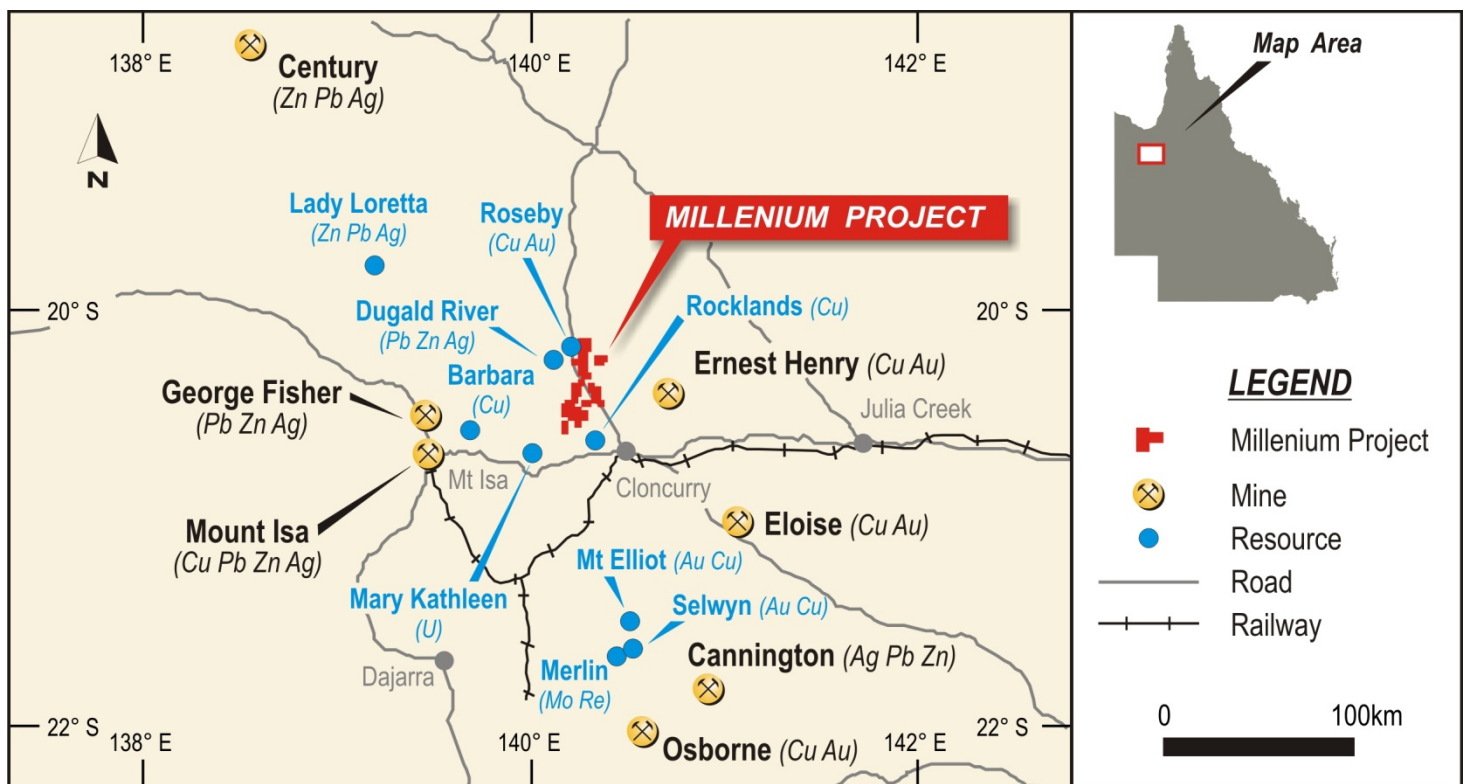
Figure 1: Location map of the granted exploration tenements in the prolific Mt Isa district, NW Queensland. The Millenium project covers the north-northwest trending Corella Fault trend and is close to several recent discoveries at Roseby, Dugald River and Rocklands.
