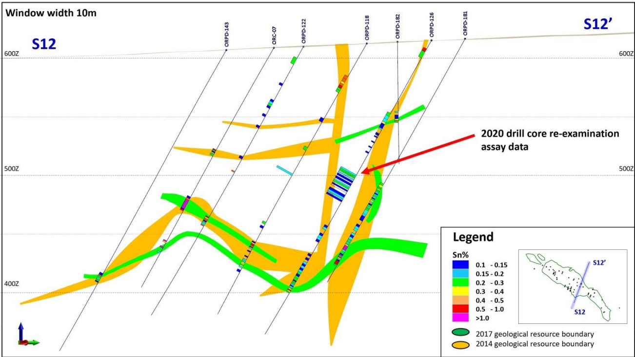
Figure 4. Cross-section S12 highlighting a significant intersection of tin mineralisation resulting from the 2020 historical drill core re-examination program at Oropesa
