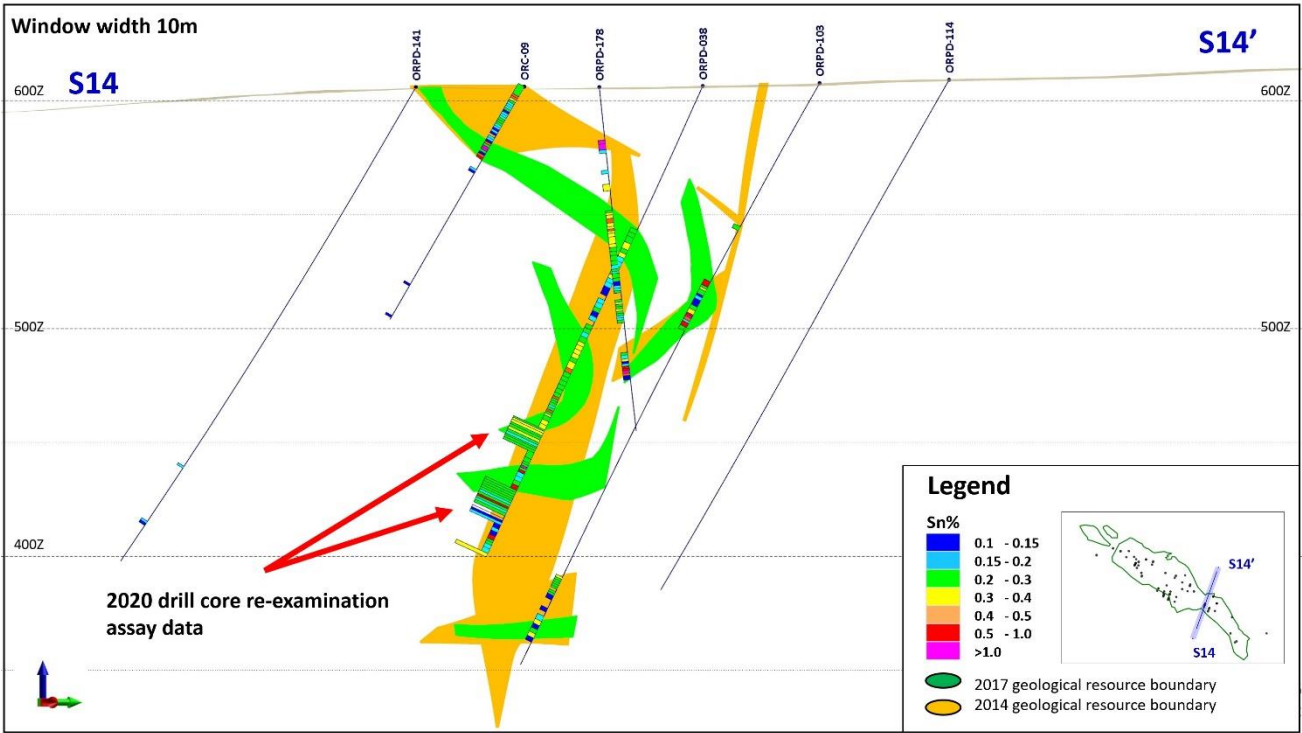
Figure 5. Cross-section S14 highlighting a significant intersection of tin mineralisation resulting from the 2020 historical drill core re-examination program at Oropesa
