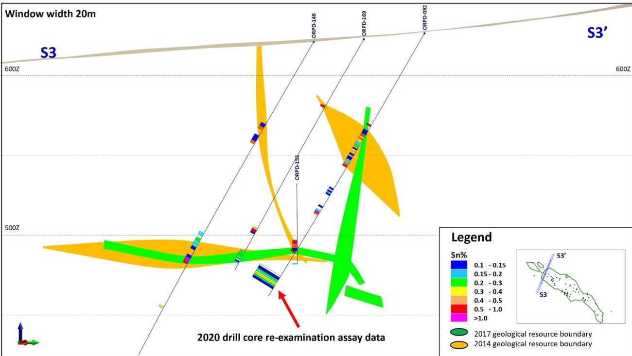
Figure3. Cross-section S3 highlighting a significant intersection of tin mineralisation resulting from the 2020 historical drill core re-examination program at Oropesa
