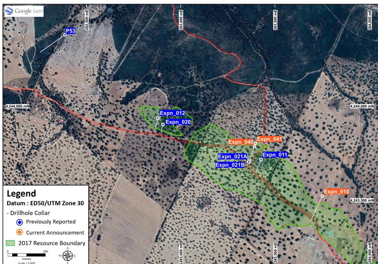
Figure 1. Location of drill holes with assay data as at 20 January 2021, from the exploration drilling program at the Oropesa Tin Project, Spain
