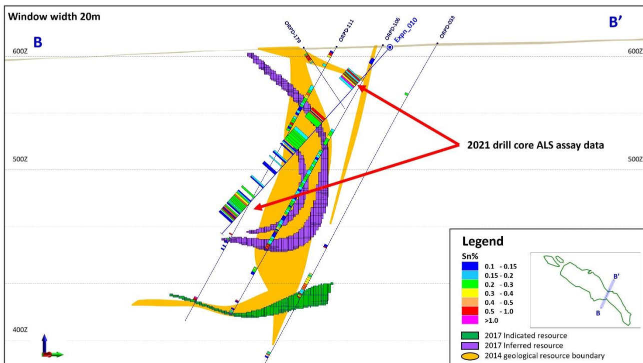
Figure 2. Oropesa 2021 resource conversion infill diamond drilling, Expn_010.
