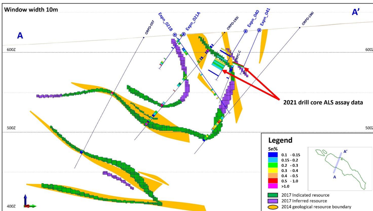
Figure 3. Oropesa 2021 resource conversion infill diamond drilling, Expn_040 & Expn_041.
