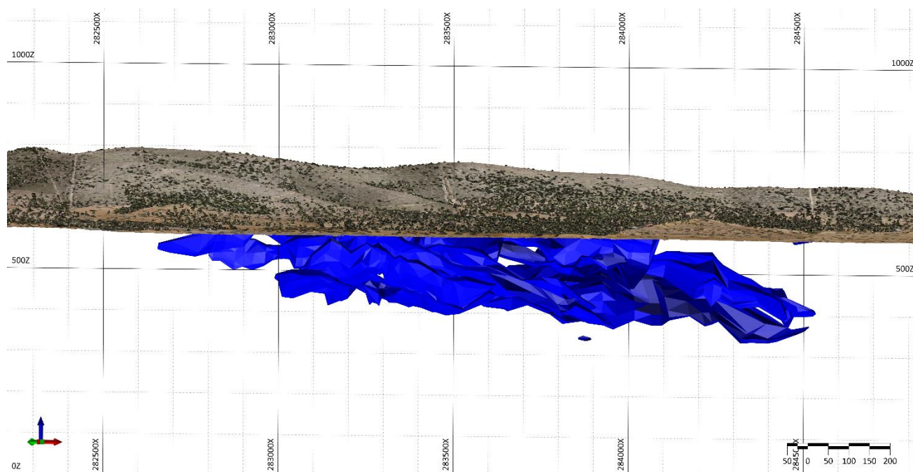
Figure 2. Oropesa Resource Model section with topography
