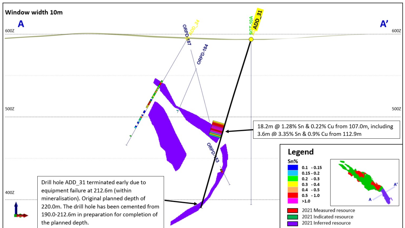
Figure 1. Section depicting drill hole ADD_31 from the 2022 Infill Drilling Program where the main aim is to upgrade the Inferred Mineral Resources within the US$30k/t pit shell into a higher confidence Mineral Resource category.
