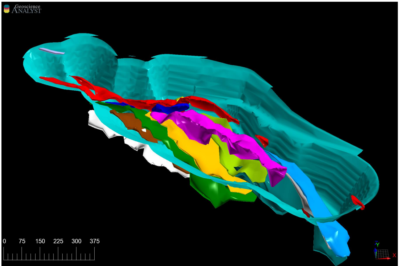
Figure 3. 2023 DFS pit shell (looking north) with the 2021 Mineral Resource Model displayed.
