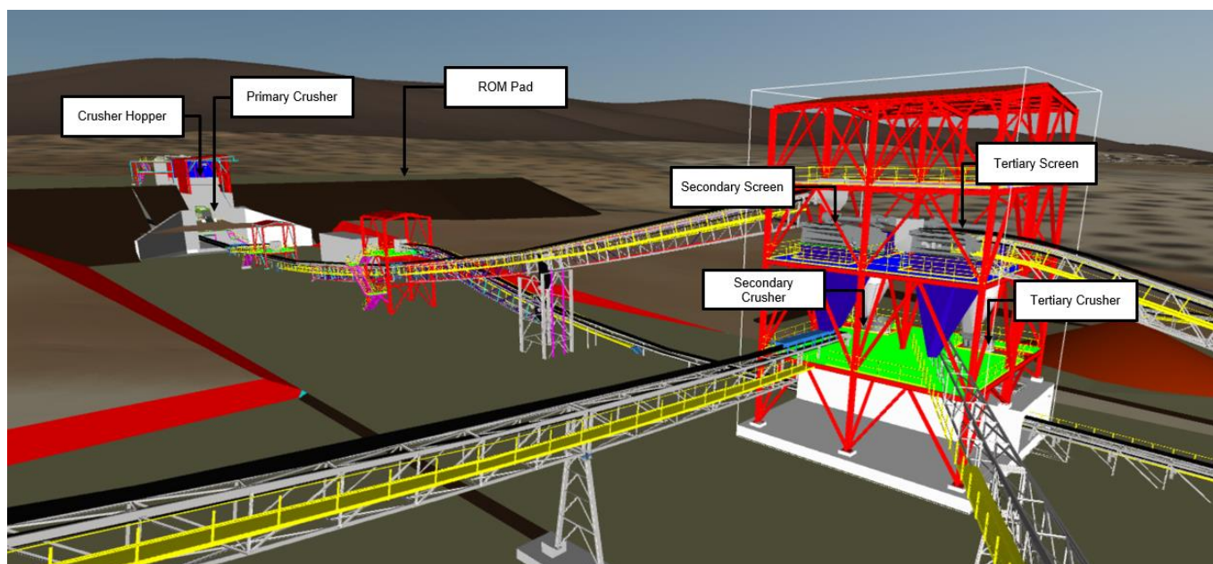
Figure 3. Crushing and Screening Circuit
