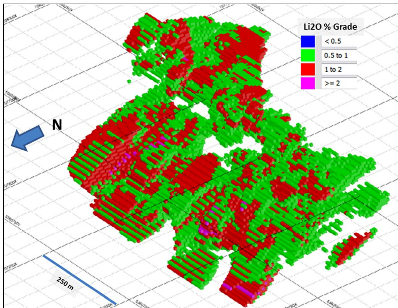
Figure 3: Lithium solid outlining the Li 2 O grade distribution throughout the deposit
