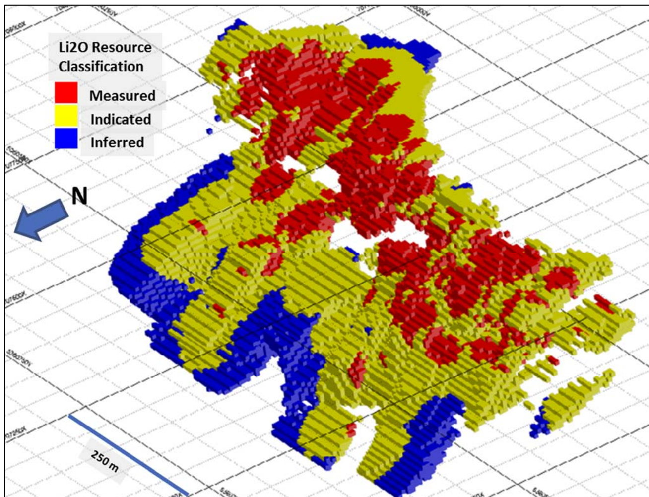
Figure 2: Lithium solid demonstrating the distribution of Measured, Indicated and Inferred Mineral Resource categories. Note the high level of Measured Resource near the surface
