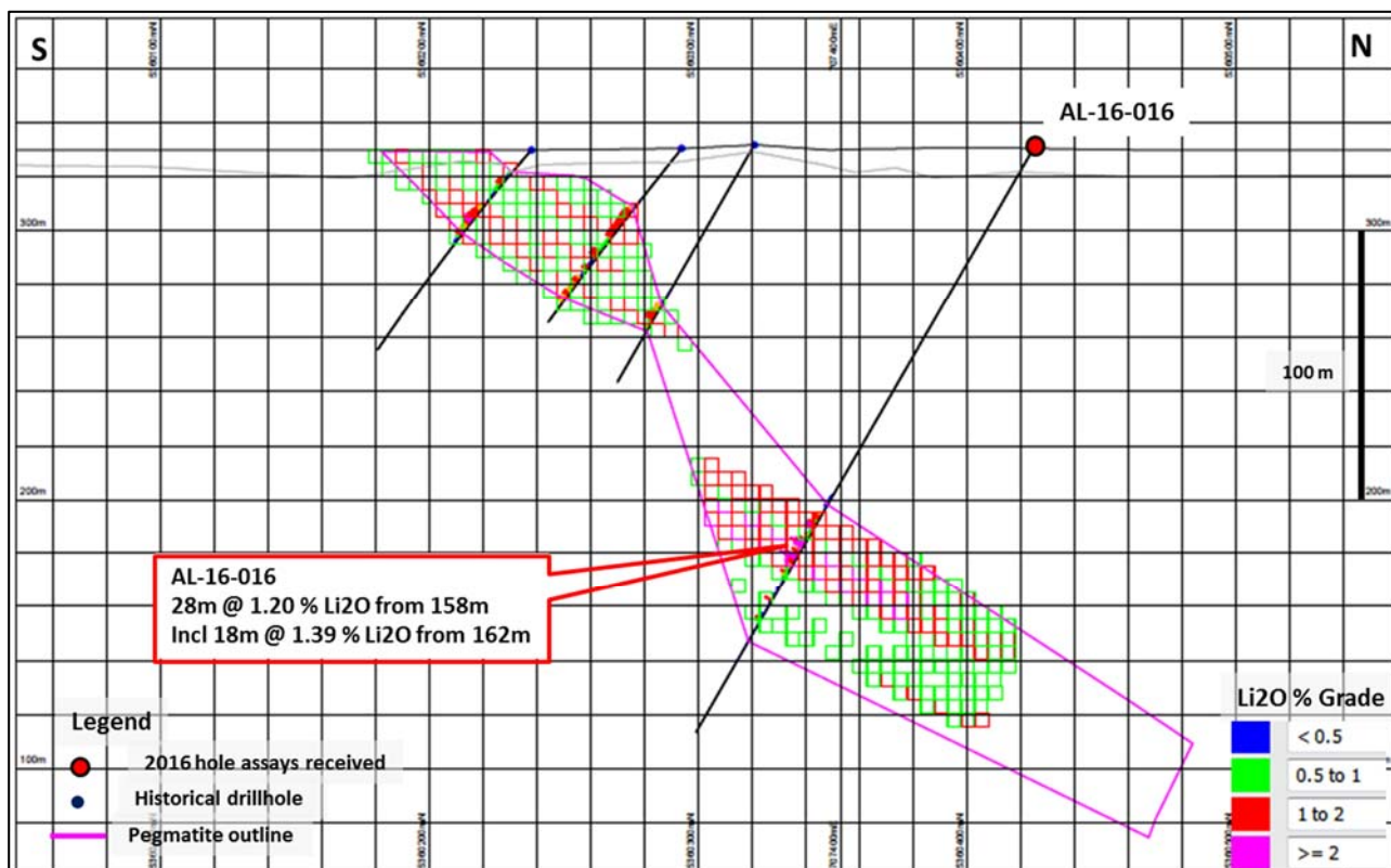
Figure 6: Section 3 looking west
