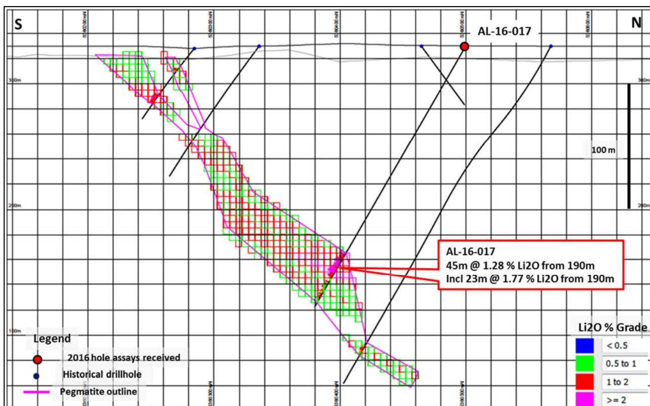
Figure 7: Section 4 looking west
