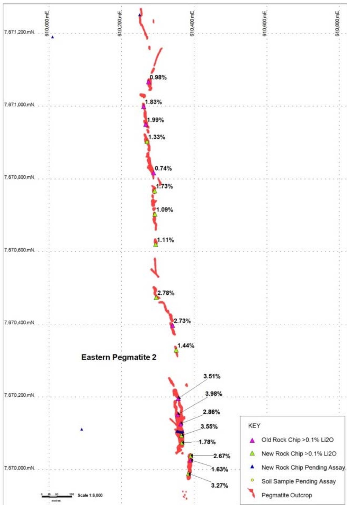
Figure 2: Eastern No.2 Pegmatite – detail of mapping and rock sampling
