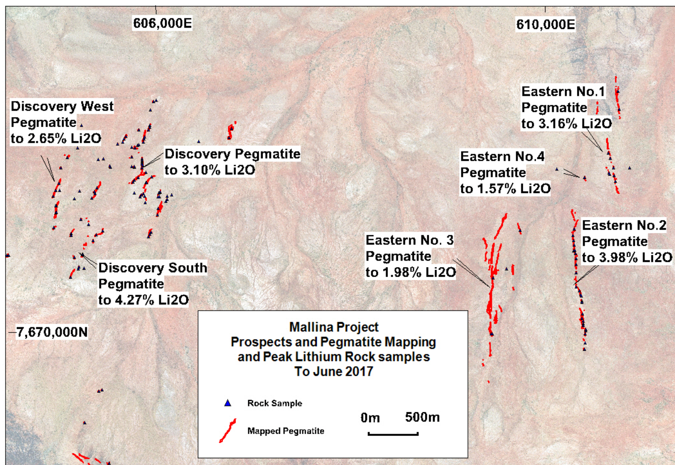
Figure 1: Location of the Mallina Spodumene Pegmatites
