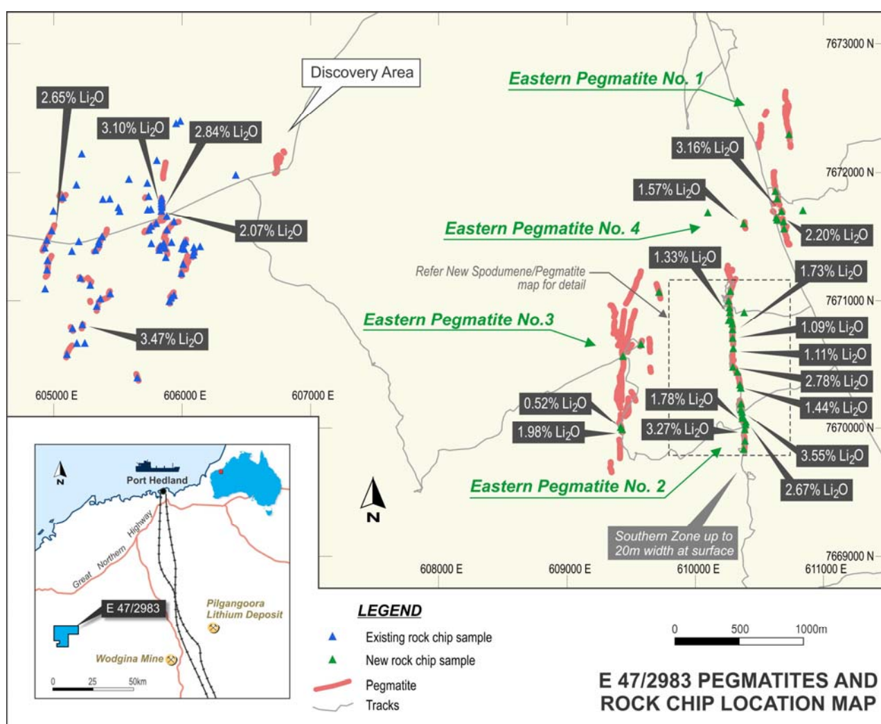
Figure 1: Mallina Project with Pegmatites and rock samples above 0.4% Li 2 O
