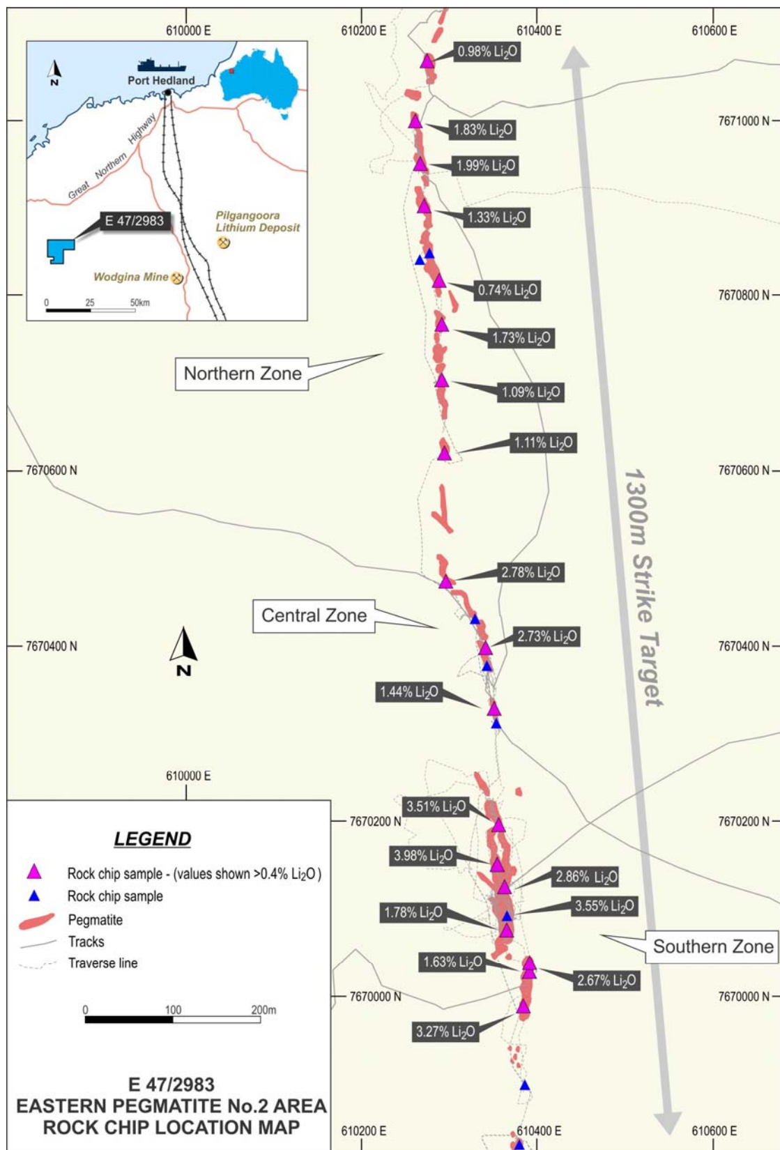
Figure 2: Eastern No.2 Pegmatite and Rock Samples over 0.4% Li 2 O
