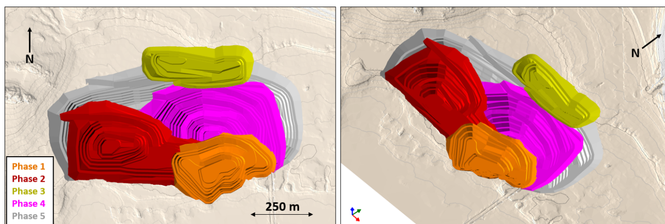
Figure 7: Schematics demonstrating the planned mining phases
