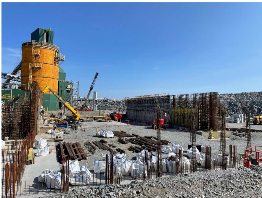
Figure 1 North American Lithium – Crushed Ore Dome side wall construction
