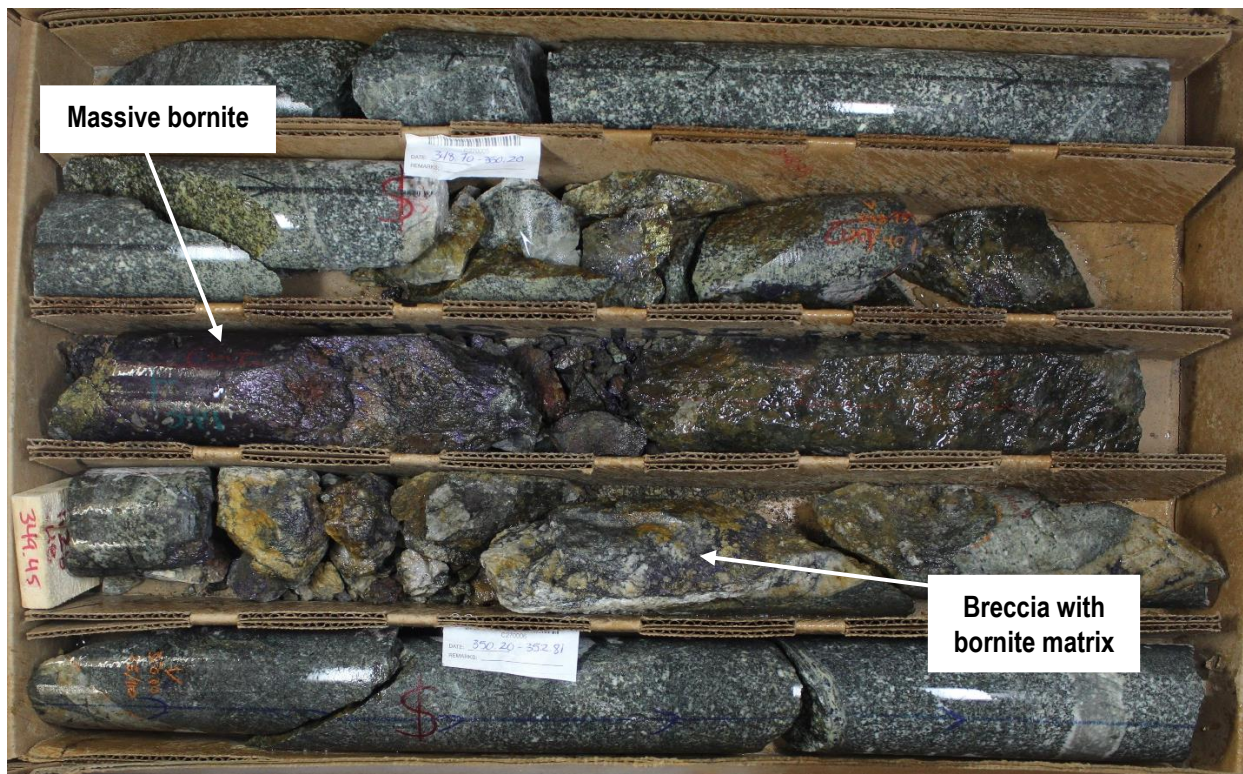
Figure 3 High-grade bornite-chalcopyrite mineralisation hosted by a vein-breccia within the Leatherwood intrusive (Hole WT-20-10, 349m downhole depth)
