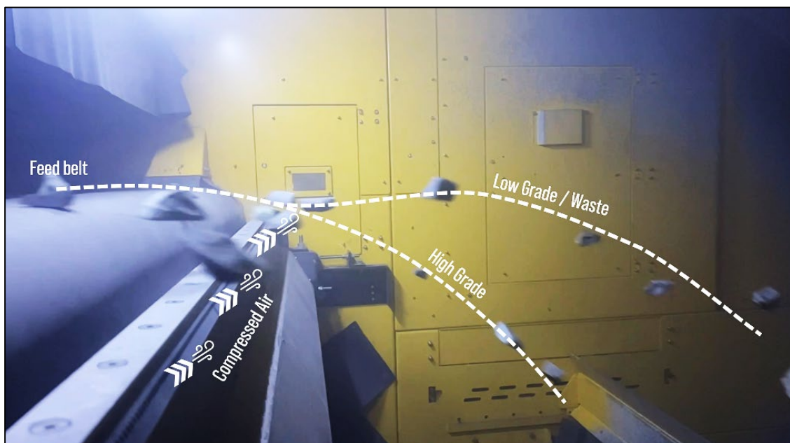
Figure 4 – Ore Sorting in progress of Oracle Ridge Mineralisation, with process shown how compressed air sorts rocks samples off a conveyor belt.
