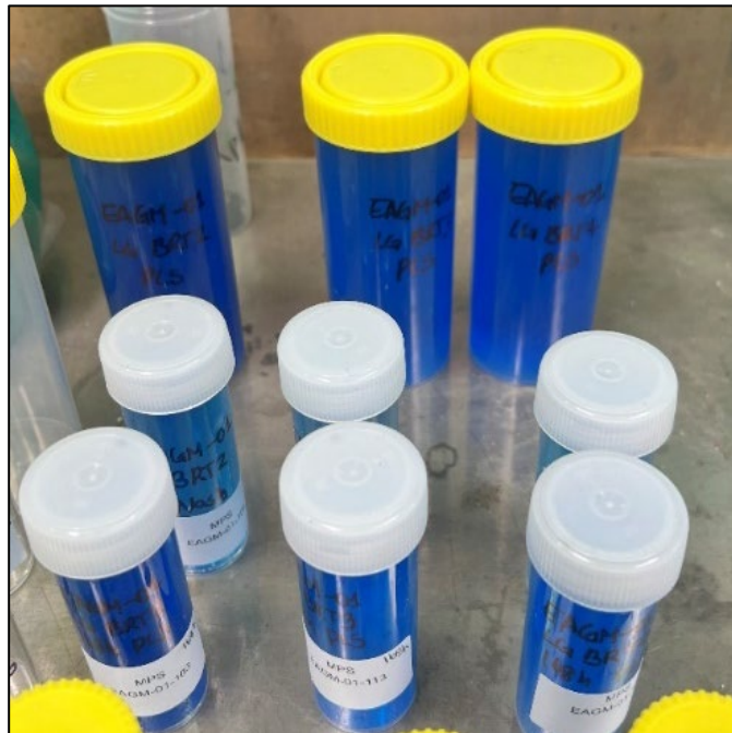
Figure 5 – Copper rich solution (copper glycinate) following bottle roll leach testwork
