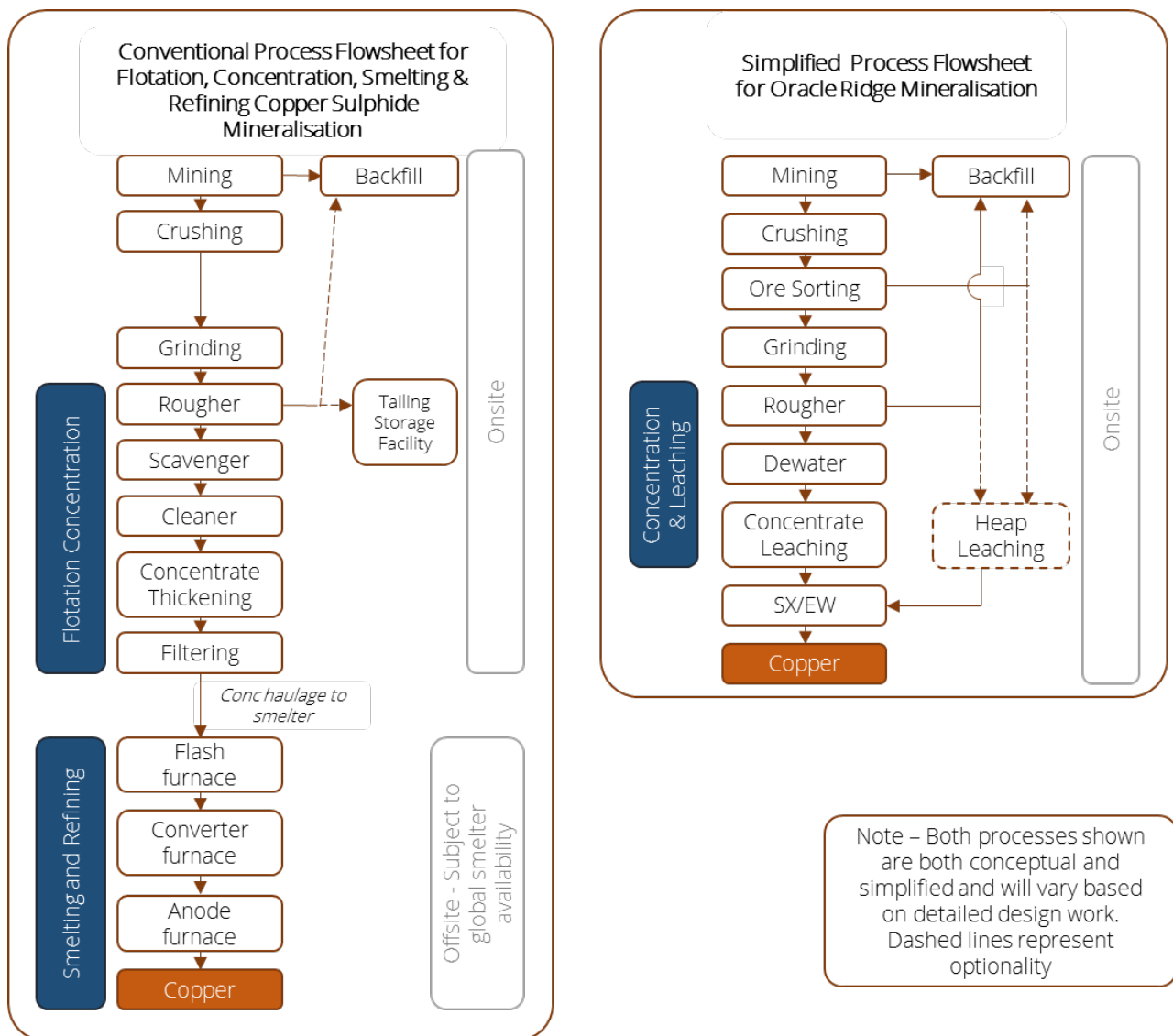
Figure 2 – Conceptual processing flowsheet for the production of LME grade copper at Oracle Ridge. Note, this is a conceptual flow sheet only which has not been economically or technically evaluated as part of any formal study.
