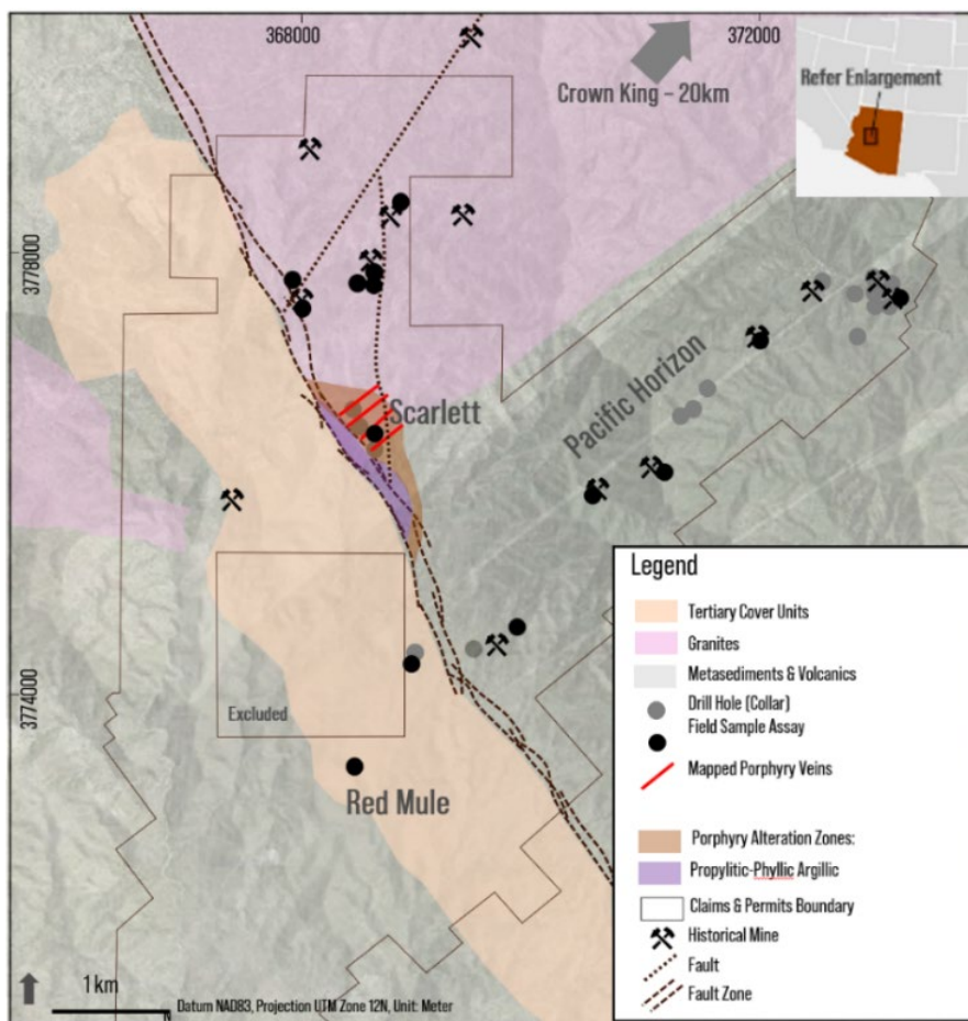
Figure 2 – Geology map showing the Silver Mountain Project showing surface alteration and veining at Scarlett prospect where porphyry targets have been identified by recent geophysical surveys (refer to ASX announcement dated 31 July 2024)
