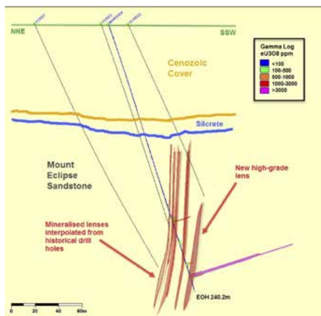
Figure 5 - Cross section (NNE to SSW) through the Malawiri prospect showing the trace of hole MARD004 with accompanying gamma downhole eU_3O_8 histogram, colour-coded for grade. Drill traces of the nearby historical holes GCRD7, 3 and 22 are also shown, together with the interpolated position of previously known mineralised lenses. A new, deeper, high-grade lens was discovered in MARD004. The unconformity between the Cenozoic cover and Mt Eclipse sandstone is shown in orange; the silcrete contact zone was probably an old land surface.
