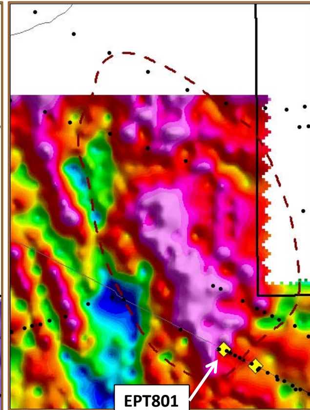
Gravity
