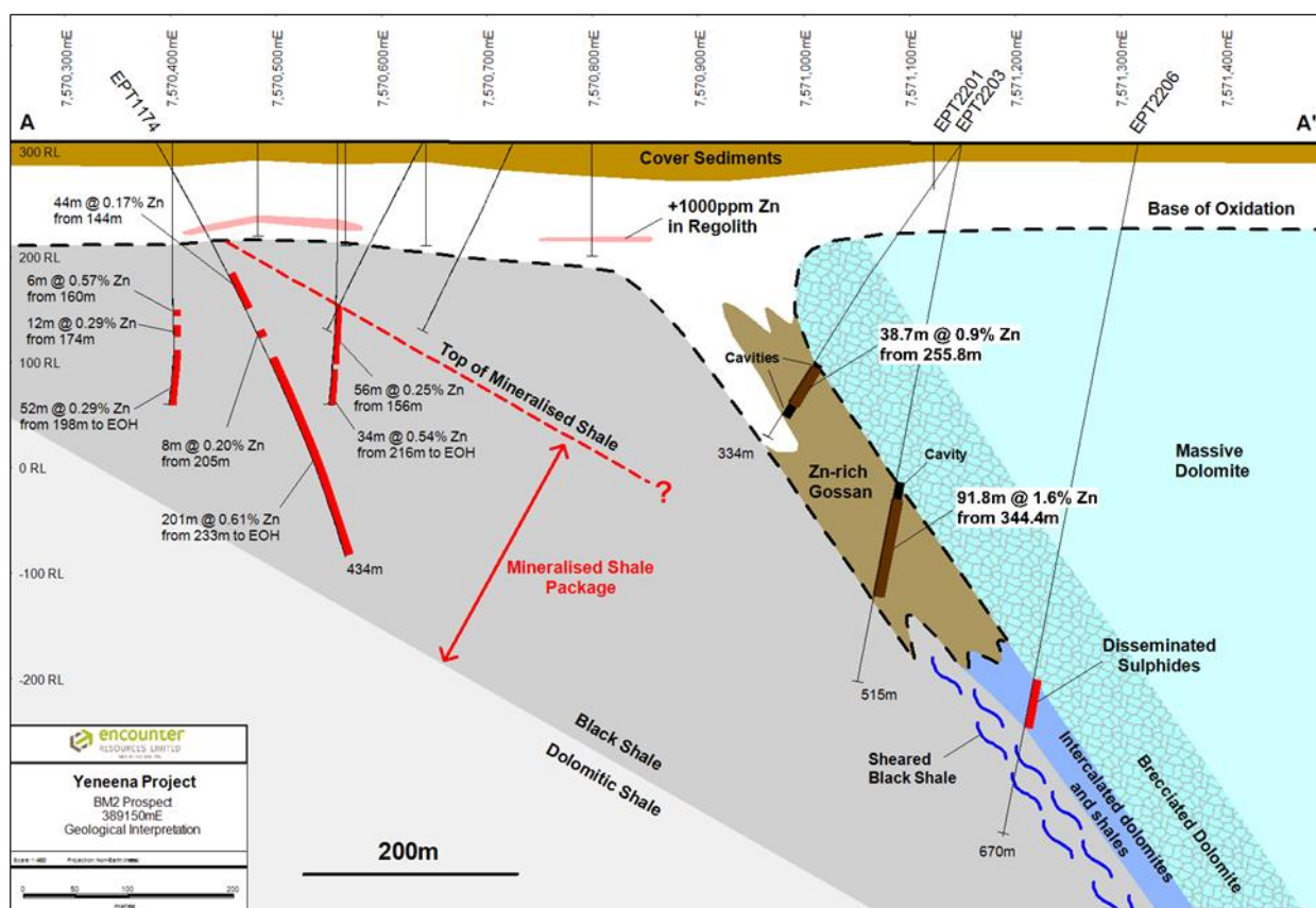
Figure 3: Cross Section 389150mE (A-A') – Millennium
