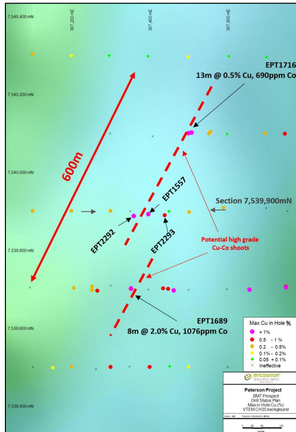
Figure 10: Drill Status plan and Max Cu in hole – BM7 Prospect (VTEM ch35 background)
