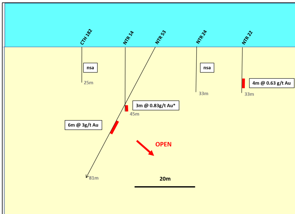
Figure 9: Schematic cross section C-C'' high grade area, Fold Closure Prospect (Horizontal: Vertical scale = 1:1)
