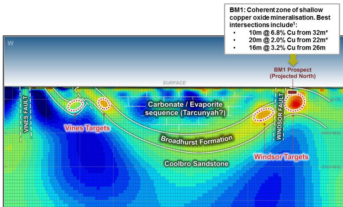
Figure 2. MT section – Vines Fault to BM1. Showing interpreted geology and the Vines and Windsor Targets
