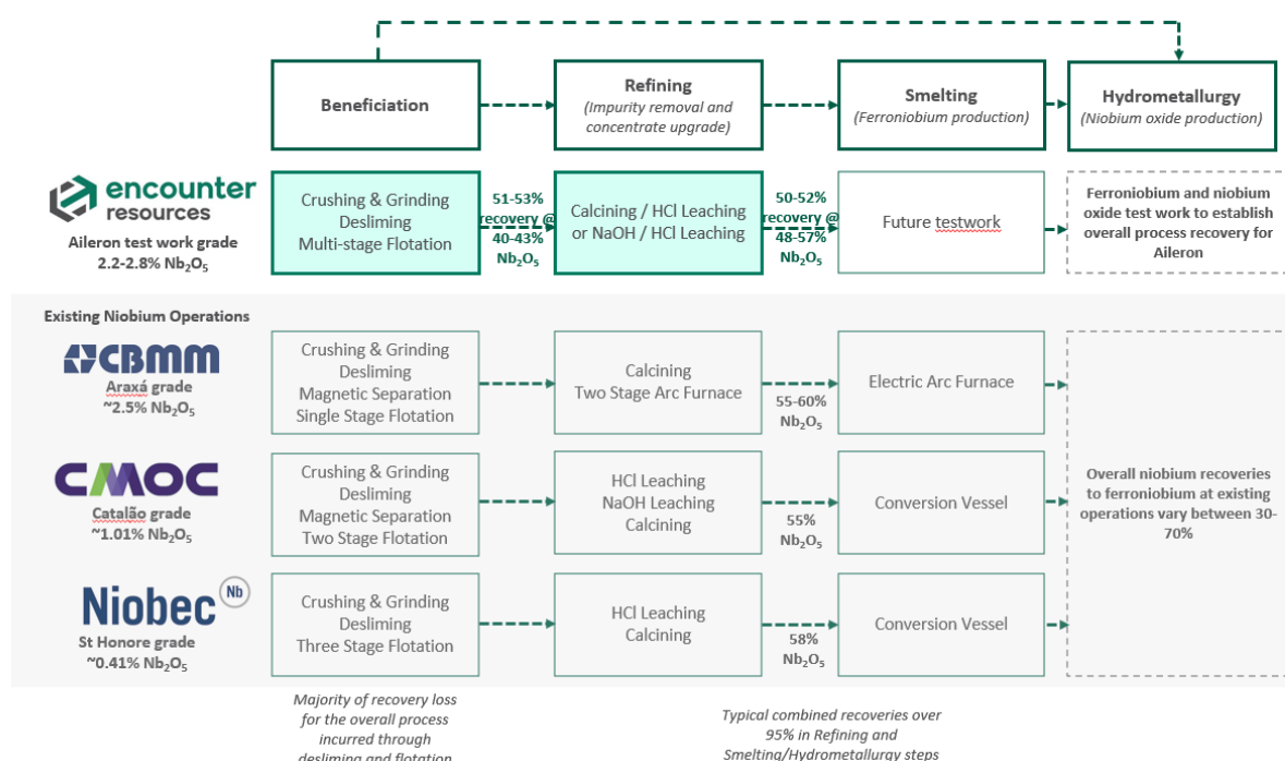
Figure 1 – Process flow sheet summary comparison to existing niobium operations 1,2,3,4,5
