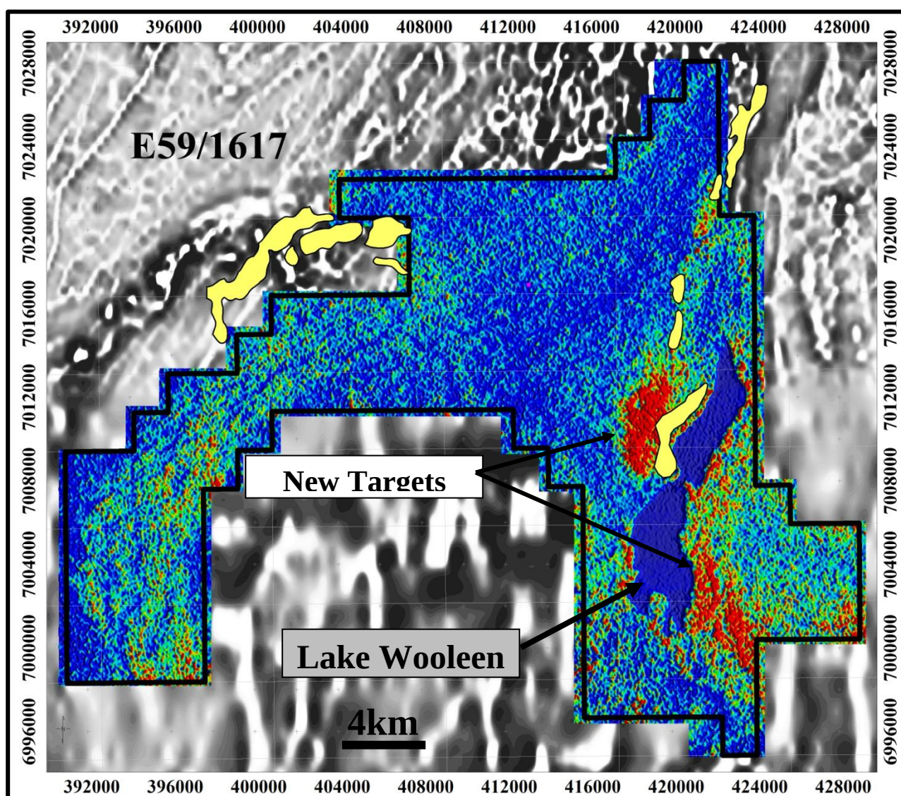
Figure 3: E59/1617 - Uranium Channel Response over TMI Aeromagnetics (GSWA mapped calcrete shown in yellow polygons)
